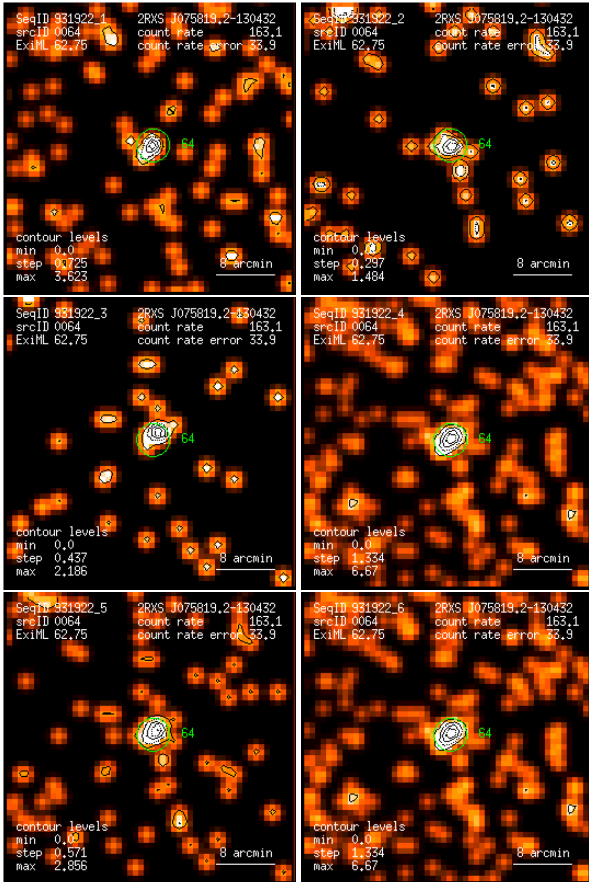
Figure 64: RASS 931922: detection 0064: band rate images, Gaussian filter: (1) PSPC channels 11 – 41, (2) 52 – 90, (3) 91 – 201, (4) 11 – 235, (5) 52 – 201, (6) 11 – 201. Broad band rates in counts/ks. Band rate contour levels in counts/ks/arcmin 2 .
