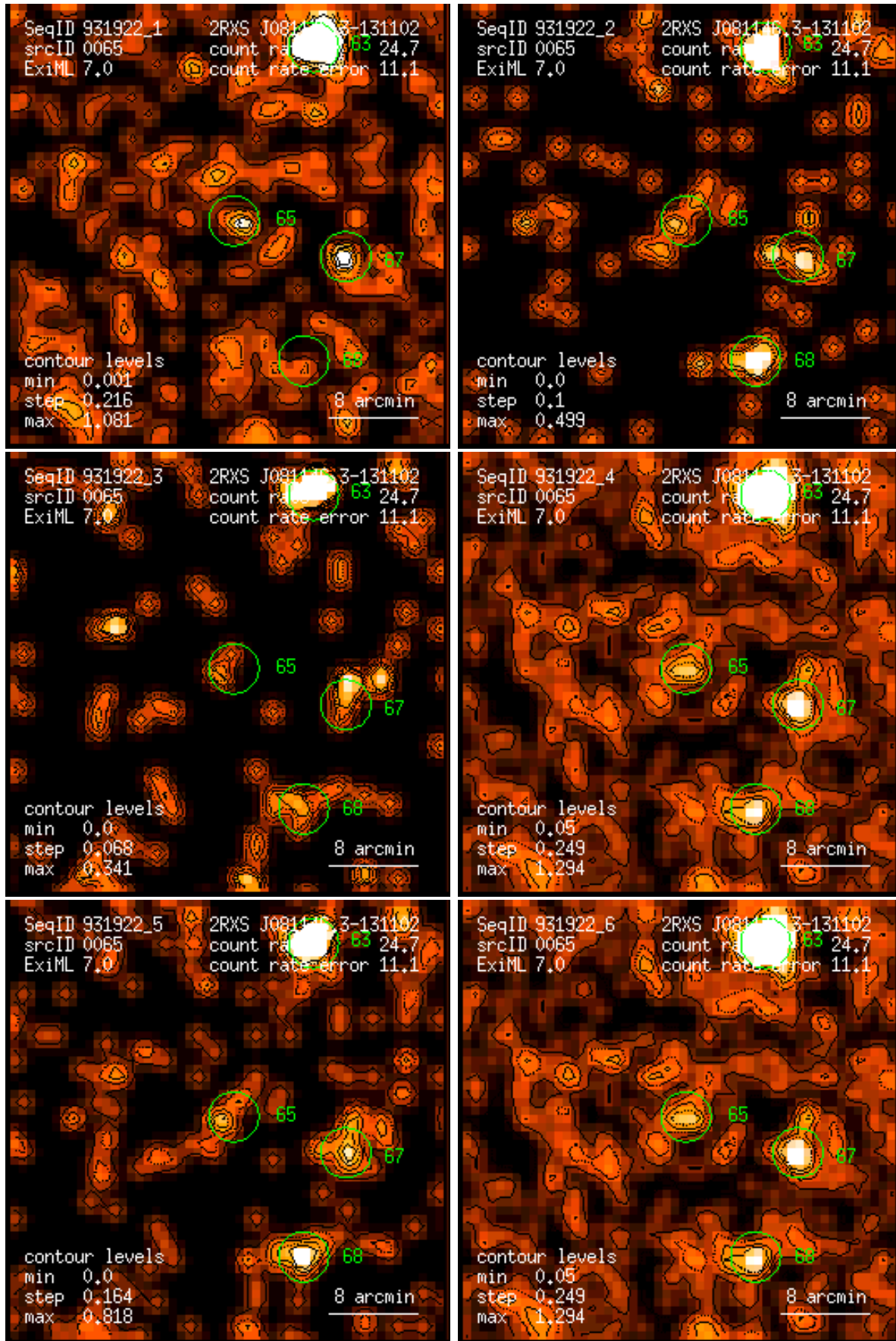
Figure 65: RASS 931922: detection 0065: band rate images, Gaussian filter: (1) PSPC channels 11 – 41, (2) 52 – 90, (3) 91 – 201, (4) 11 – 235, (5) 52 – 201, (6) 11 – 201. Broad band rates in counts/ks. Band rate contour levels in counts/ks/arcmin 2 .
