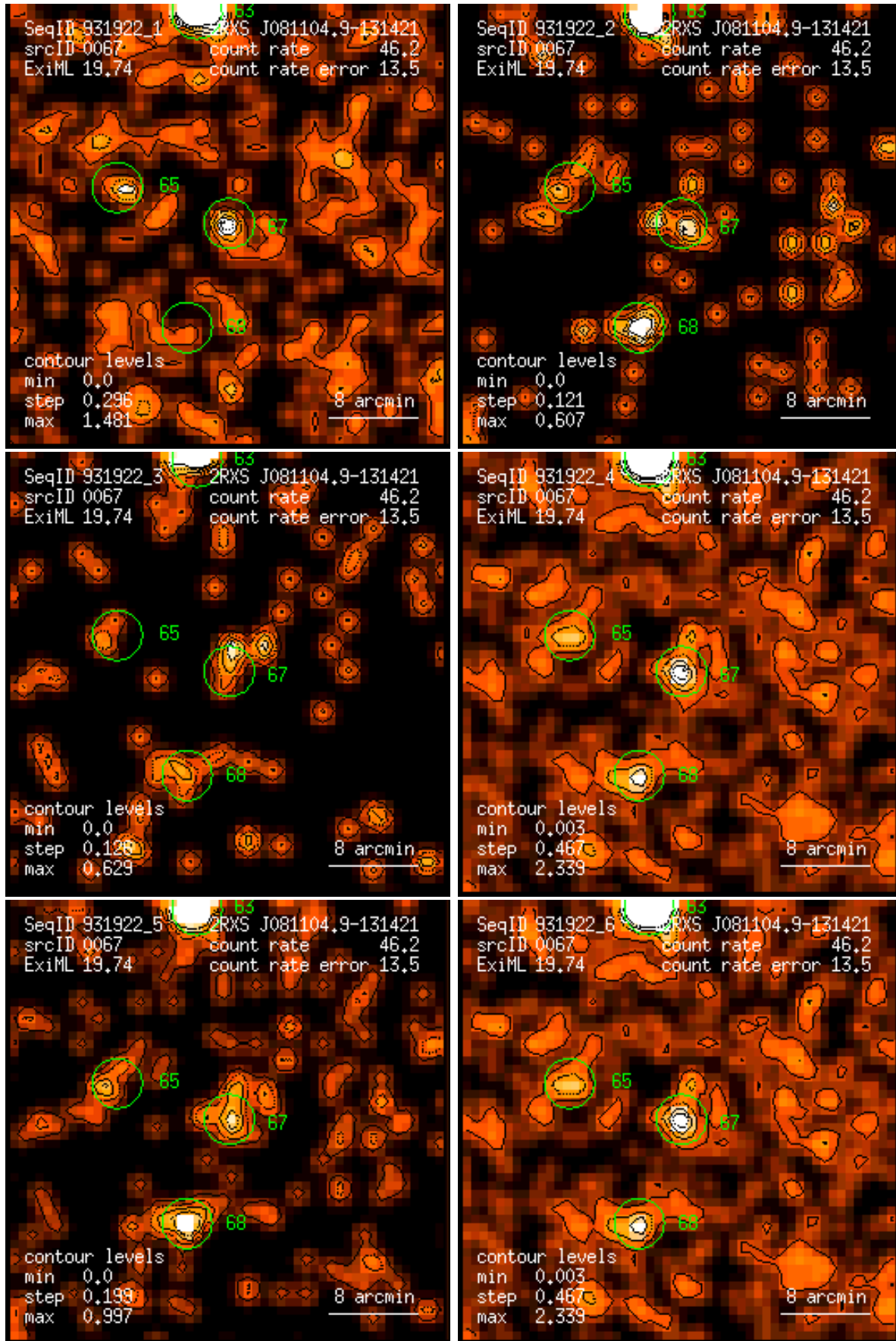
Figure 67: RASS 931922: detection 0067: band rate images, Gaussian filter: (1) PSPC channels 11 – 41, (2) 52 – 90, (3) 91 – 201, (4) 11 – 235, (5) 52 – 201, (6) 11 – 201. Broad band rates in counts/ks. Band rate contour levels in counts/ks/arcmin 2 .
