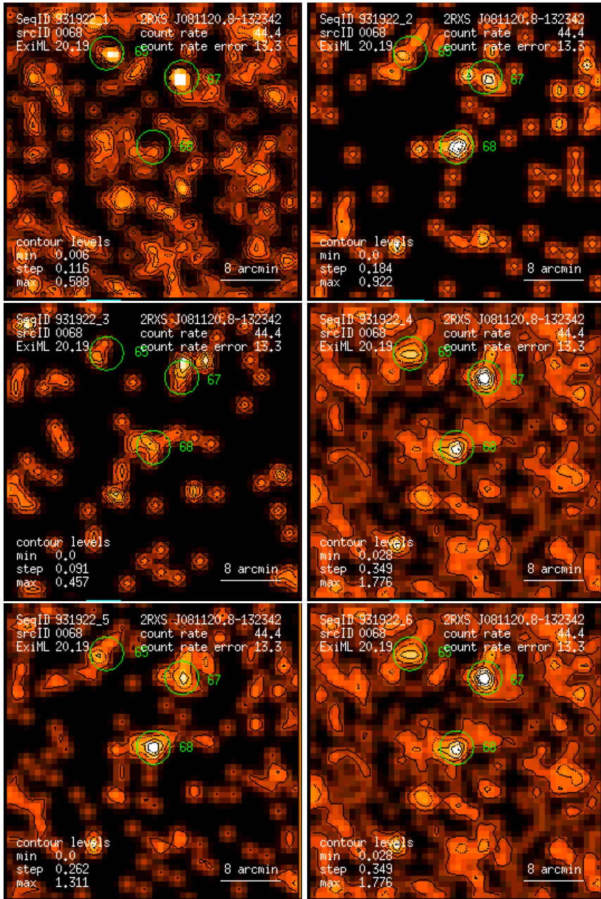
Figure 68: RASS 931922: detection 0068: band rate images, Gaussian filter: (1) PSPC channels 11 – 41, (2) 52 – 90, (3) 91 – 201, (4) 11 – 235, (5) 52 – 201, (6) 11 – 201. Broad band rates in counts/ks. Band rate contour levels in counts/ks/arcmin 2 .
