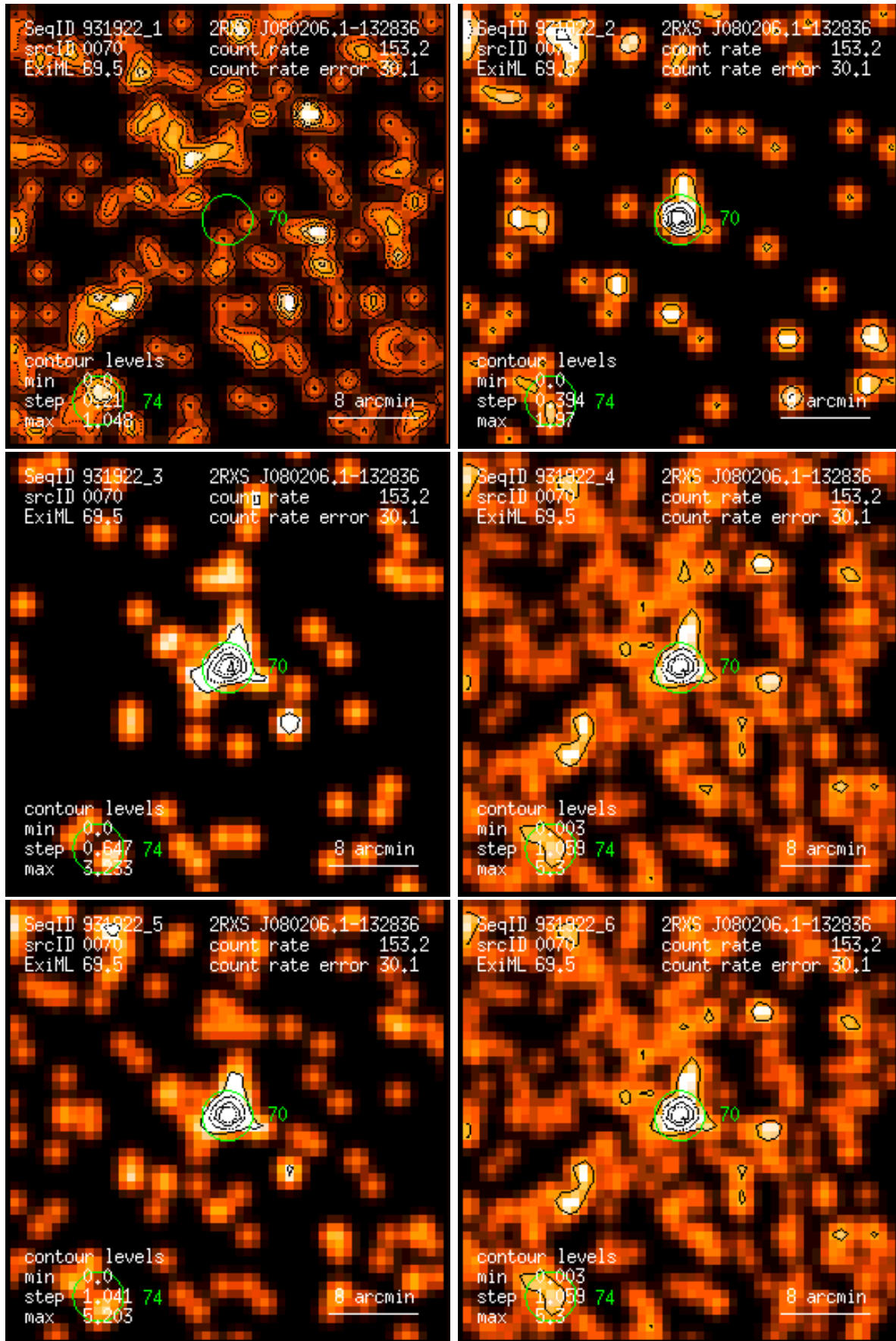
Figure 70: RASS 931922: detection 0070: band rate images, Gaussian filter: (1) PSPC channels 11 – 41, (2) 52 – 90, (3) 91 – 201, (4) 11 – 235, (5) 52 – 201, (6) 11 – 201. Broad band rates in counts/ks. Band rate contour levels in counts/ks/arcmin 2 .
