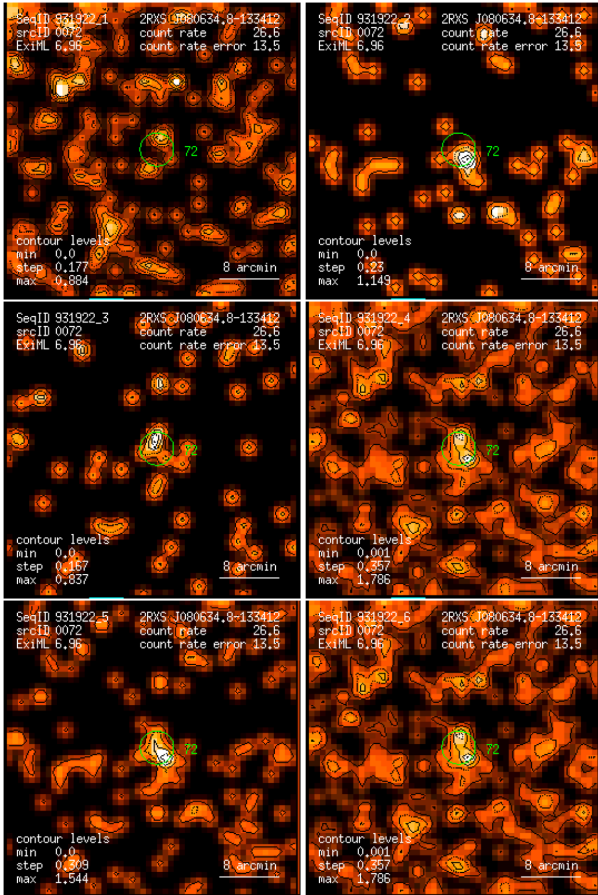
Figure 72: RASS 931922: detection 0072: band rate images, Gaussian filter: (1) PSPC channels 11 – 41, (2) 52 – 90, (3) 91 – 201, (4) 11 – 235, (5) 52 – 201, (6) 11 – 201. Broad band rates in counts/ks. Band rate contour levels in counts/ks/arcmin 2 .
