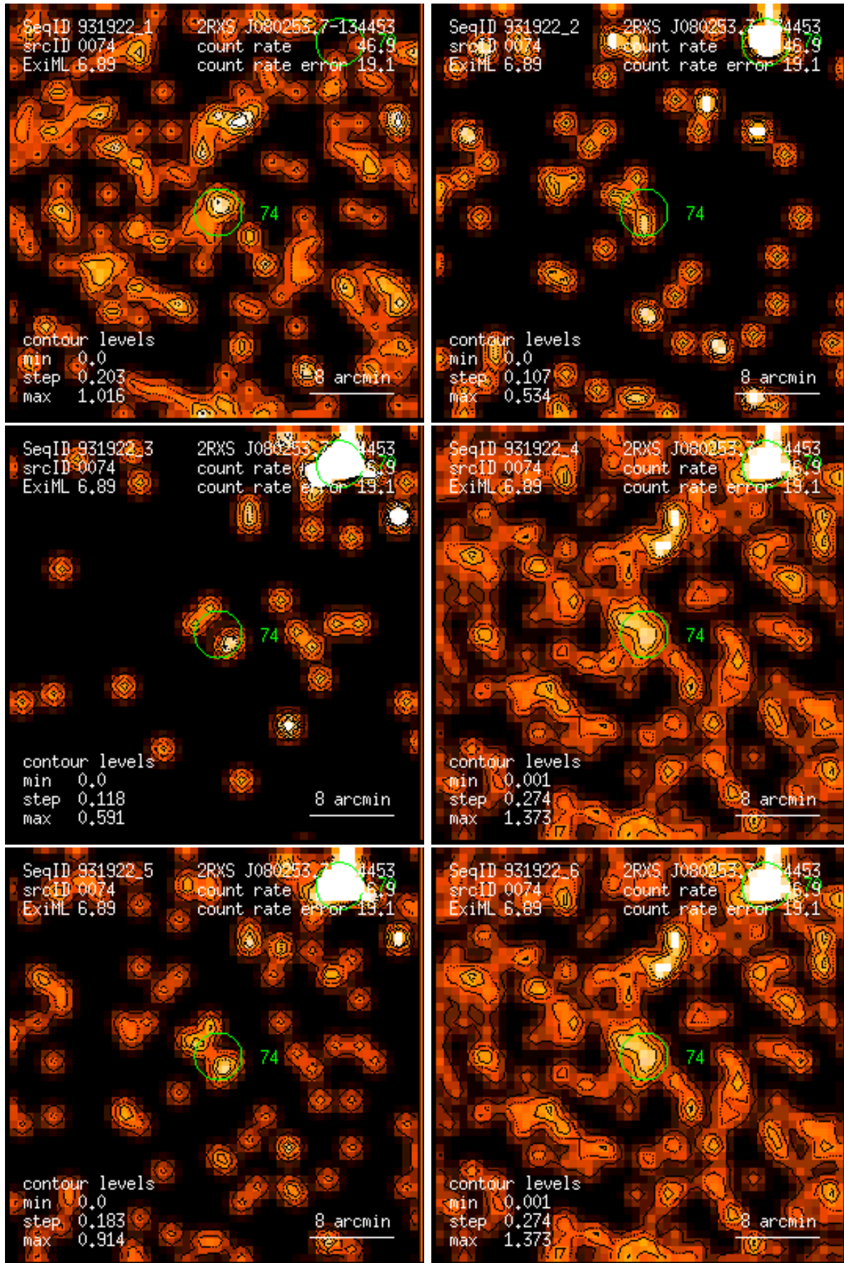
Figure 74: RASS 931922: detection 0074: band rate images, Gaussian filter: (1) PSPC channels 11 – 41, (2) 52 – 90, (3) 91 – 201, (4) 11 – 235, (5) 52 – 201, (6) 11 – 201. Broad band rates in counts/ks. Band rate contour levels in counts/ks/arcmin 2 .
