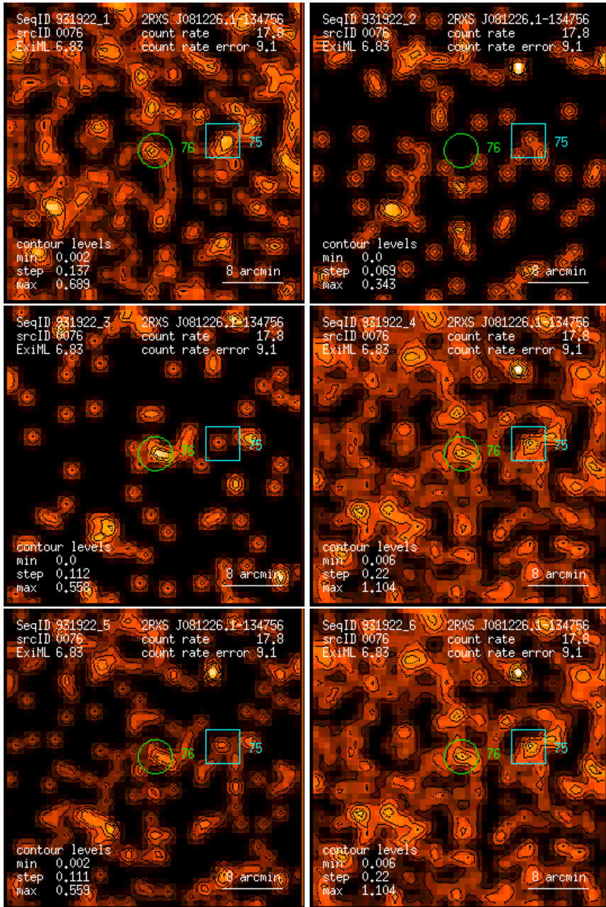
Figure 76: RASS 931922: detection 0076: band rate images, Gaussian filter: (1) PSPC channels 11 – 41, (2) 52 – 90, (3) 91 – 201, (4) 11 – 235, (5) 52 – 201, (6) 11 – 201. Broad band rates in counts/ks. Band rate contour levels in counts/ks/arcmin 2 .
