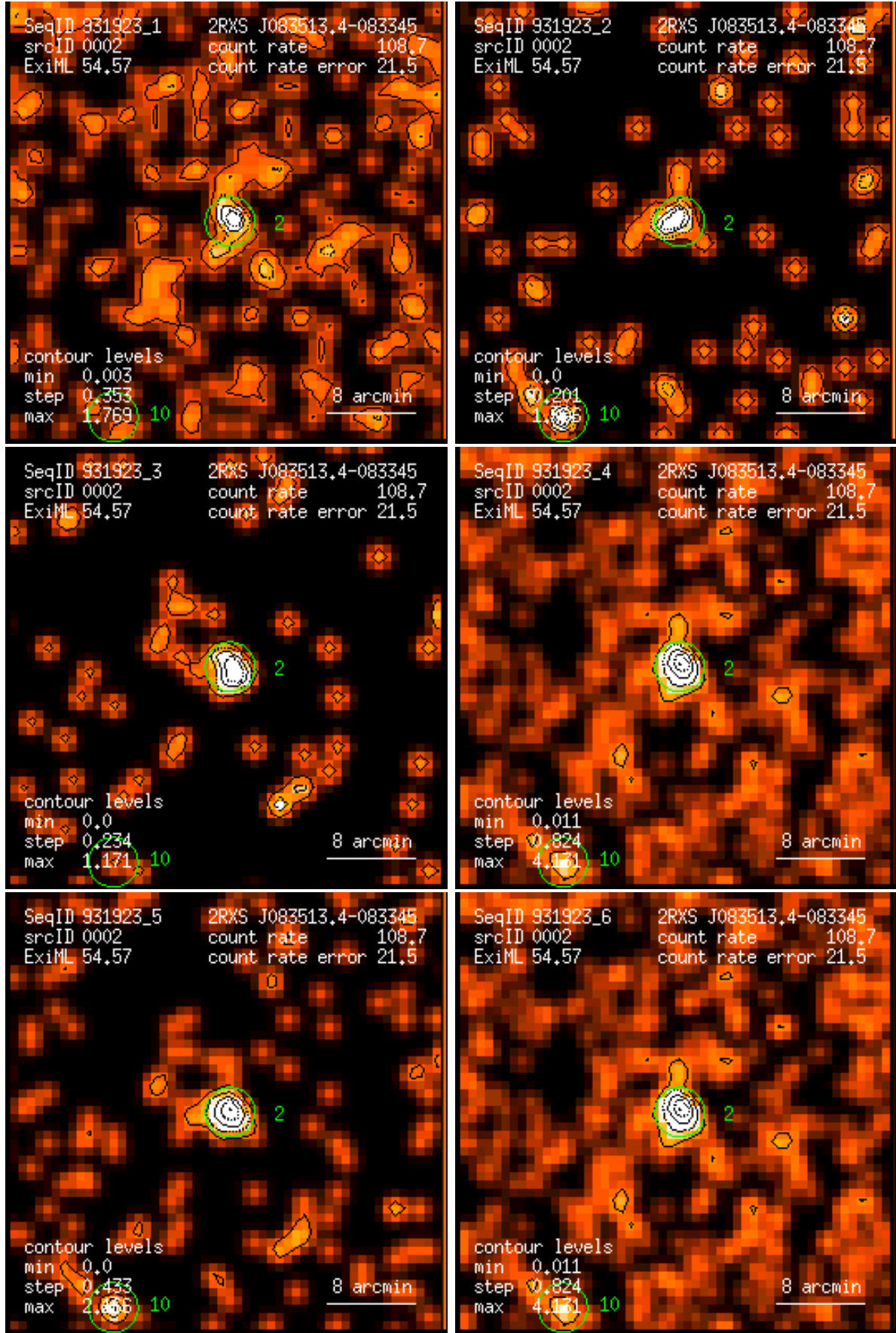
Figure 2: RASS 931923: detection 0002: band rate images, Gaussian filter: (1) PSPC channels 11 – 41, (2) 52 – 90, (3) 91 – 201, (4) 11 – 235, (5) 52 – 201, (6) 11 – 201. Broad band rates in counts/ks. Band rate contour levels in counts/ks/arcmin 2 .
