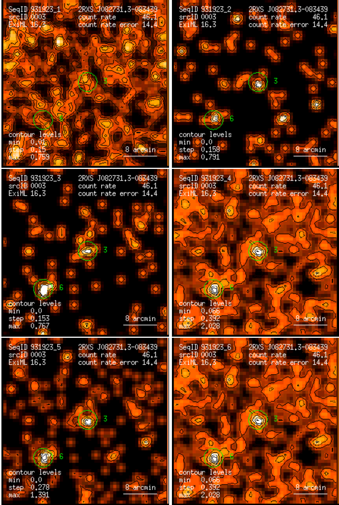
Figure 3: RASS 931923: detection 0003: band rate images, Gaussian filter: (1) PSPC channels 11 – 41, (2) 52 – 90, (3) 91 – 201, (4) 11 – 235, (5) 52 – 201, (6) 11 – 201. Broad band rates in counts/ks. Band rate contour levels in counts/ks/arcmin 2 .
