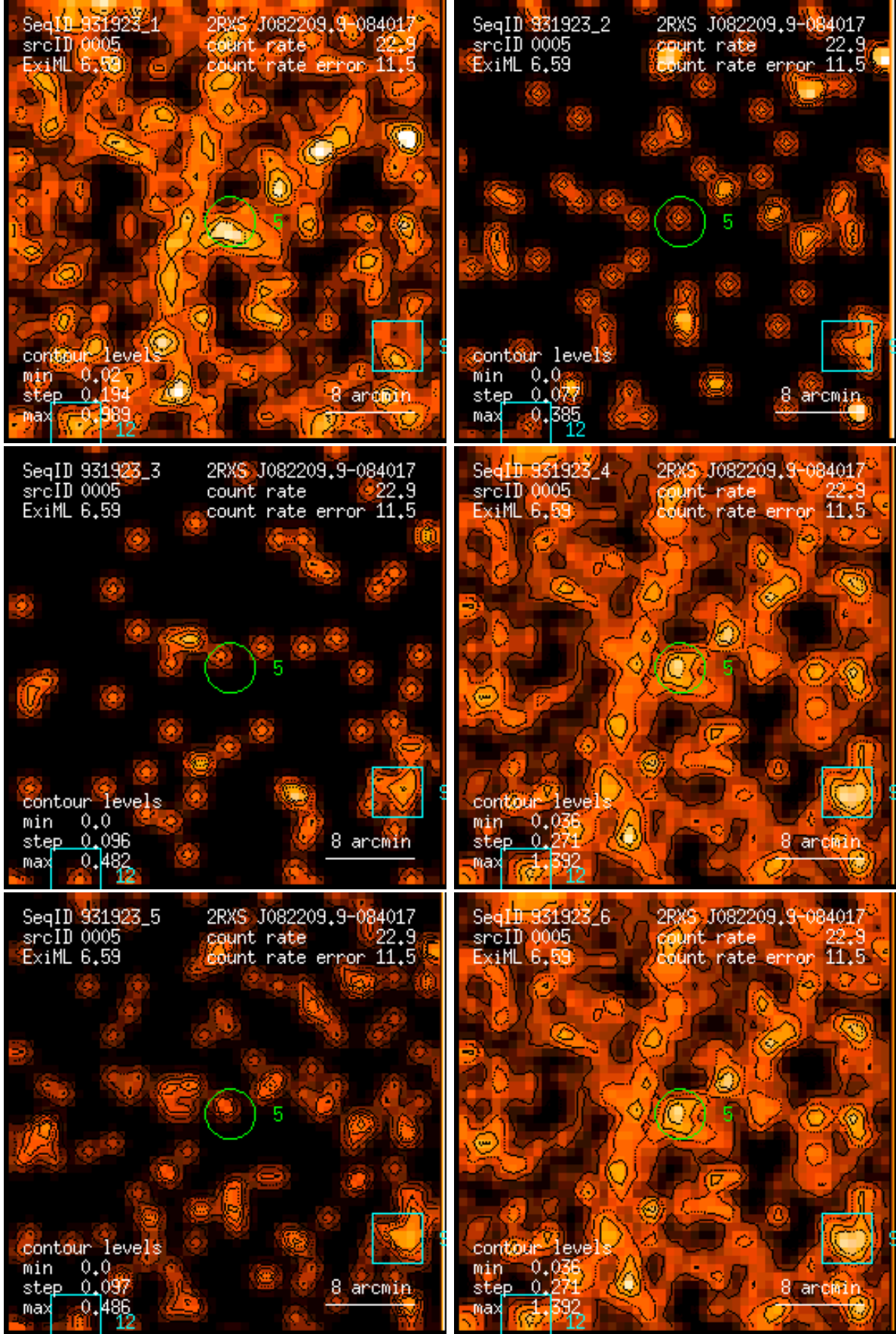
Figure 5: RASS 931923: detection 0005: band rate images, Gaussian filter: (1) PSPC channels 11 – 41, (2) 52 – 90, (3) 91 – 201, (4) 11 – 235, (5) 52 – 201, (6) 11 – 201. Broad band rates in counts/ks. Band rate contour levels in counts/ks/arcmin 2 .
