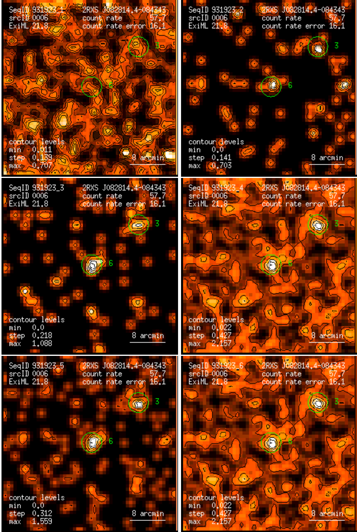
Figure 6: RASS 931923: detection 0006: band rate images, Gaussian filter: (1) PSPC channels 11 – 41, (2) 52 – 90, (3) 91 – 201, (4) 11 – 235, (5) 52 – 201, (6) 11 – 201. Broad band rates in counts/ks. Band rate contour levels in counts/ks/arcmin 2 .
