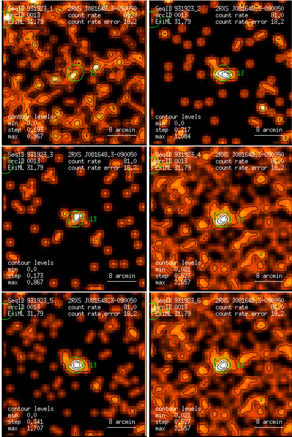
Figure 13: RASS 931923: detection 0013: band rate images, Gaussian filter: (1) PSPC channels 11 – 41, (2) 52 – 90, (3) 91 – 201, (4) 11 – 235, (5) 52 – 201, (6) 11 – 201. Broad band rates in counts/ks. Band rate contour levels in counts/ks/arcmin 2 .
