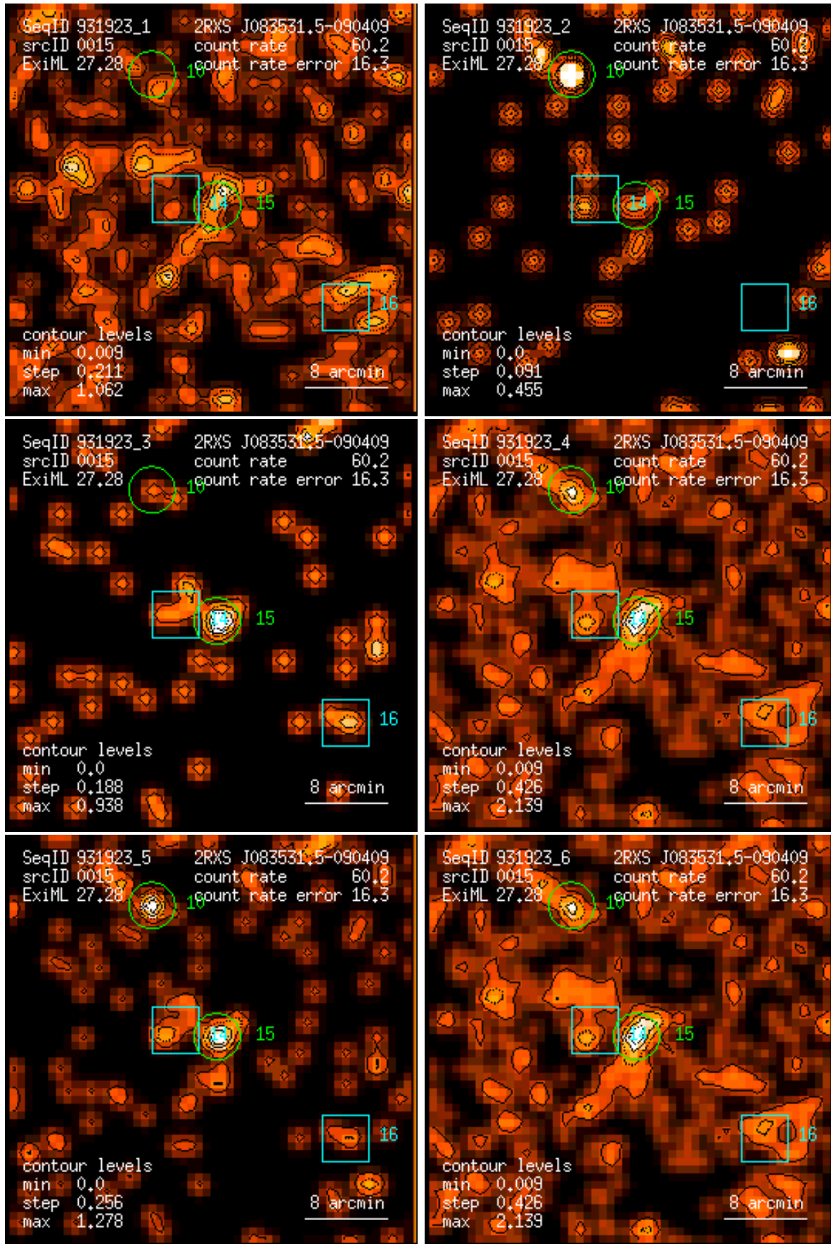
Figure 15: RASS 931923: detection 0015: band rate images, Gaussian filter: (1) PSPC channels 11 – 41, (2) 52 – 90, (3) 91 – 201, (4) 11 – 235, (5) 52 – 201, (6) 11 – 201. Broad band rates in counts/ks. Band rate contour levels in counts/ks/arcmin 2 .
