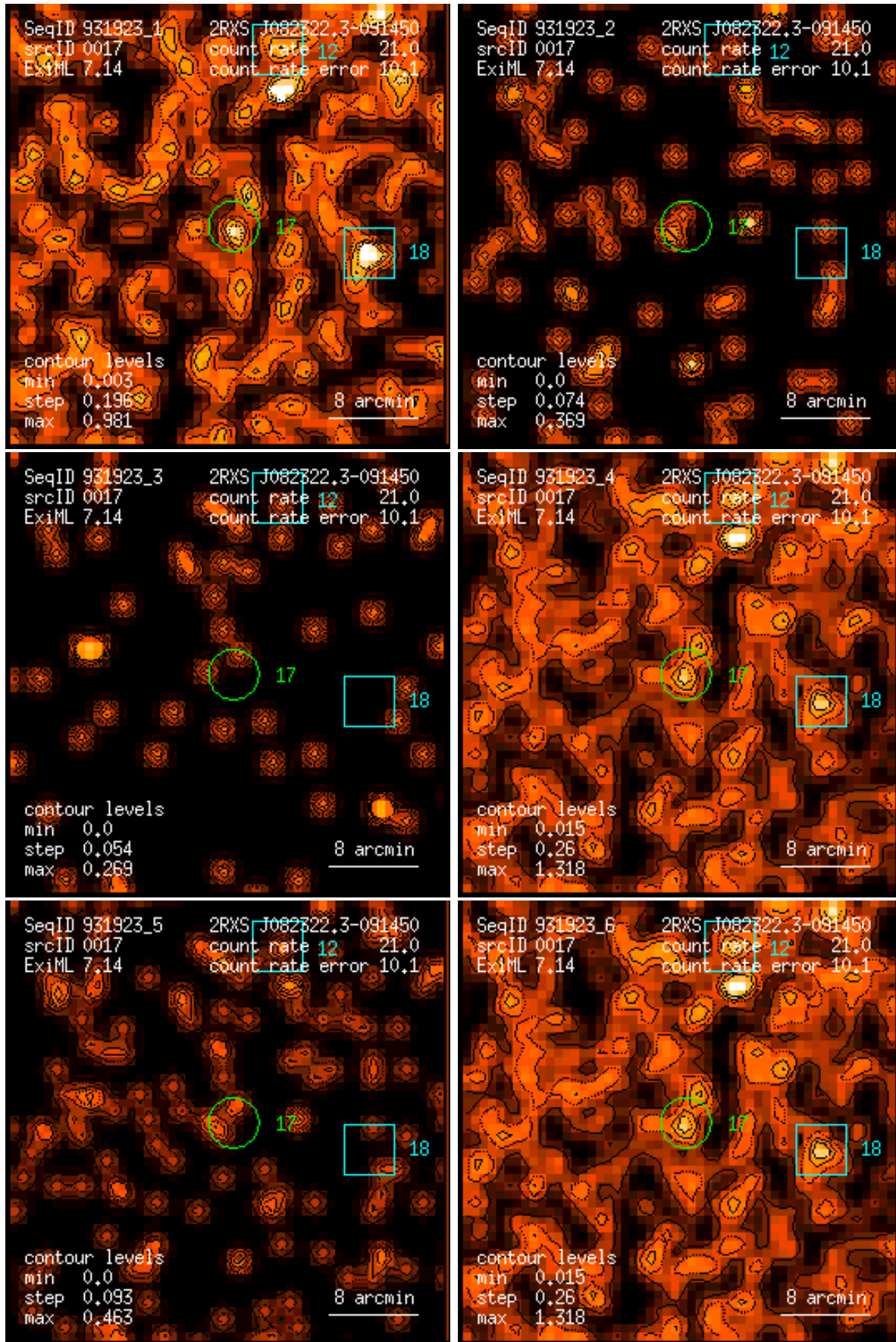
Figure 17: RASS 931923: detection 0017: band rate images, Gaussian filter: (1) PSPC channels 11 – 41, (2) 52 – 90, (3) 91 – 201, (4) 11 – 235, (5) 52 – 201, (6) 11 – 201. Broad band rates in counts/ks. Band rate contour levels in counts/ks/arcmin 2 .
