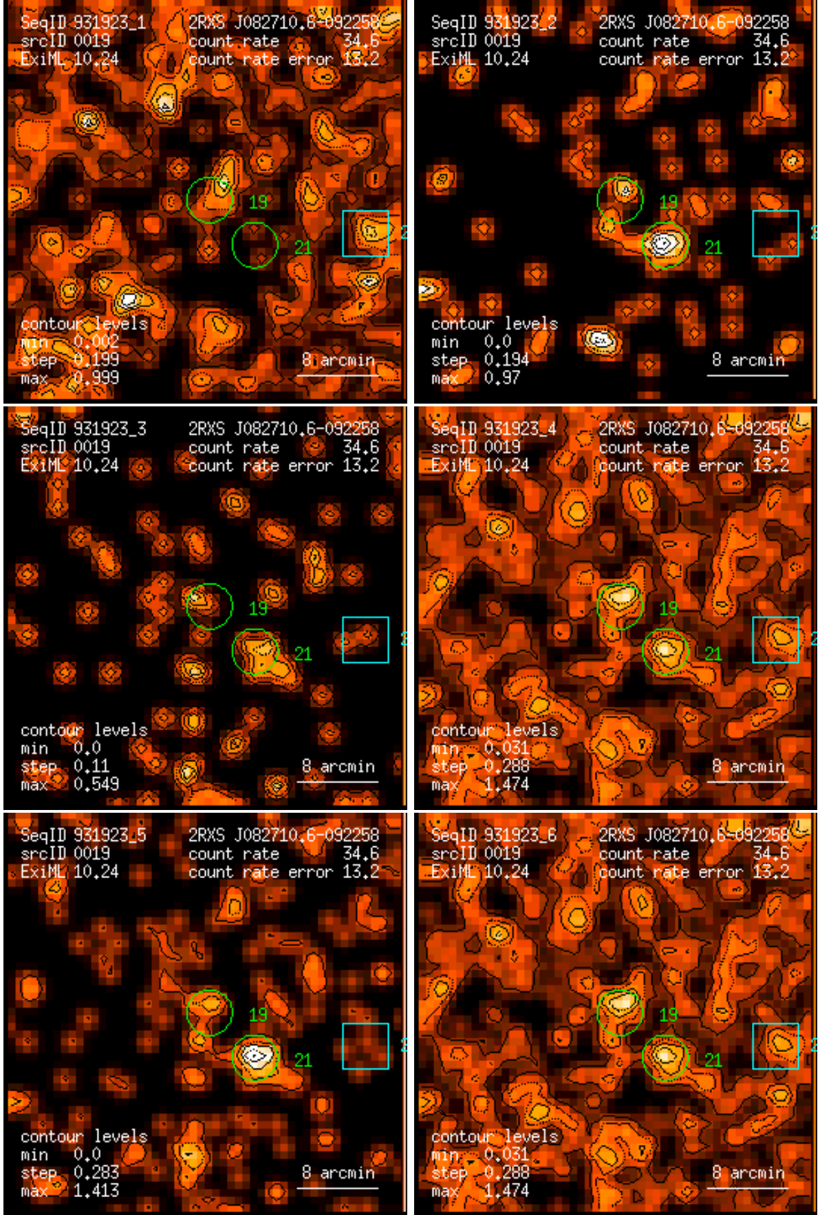
Figure 19: RASS 931923: detection 0019: band rate images, Gaussian filter: (1) PSPC channels 11 – 41, (2) 52 – 90, (3) 91 – 201, (4) 11 – 235, (5) 52 – 201, (6) 11 – 201. Broad band rates in counts/ks. Band rate contour levels in counts/ks/arcmin 2 .
