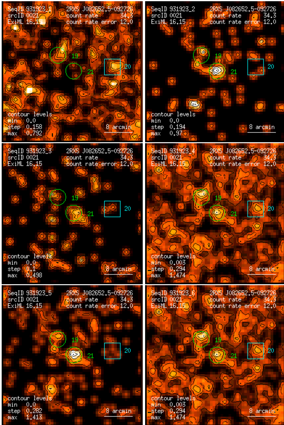
Figure 21: RASS 931923: detection 0021: band rate images, Gaussian filter: (1) PSPC channels 11 – 41, (2) 52 – 90, (3) 91 – 201, (4) 11 – 235, (5) 52 – 201, (6) 11 – 201. Broad band rates in counts/ks. Band rate contour levels in counts/ks/arcmin 2 .
