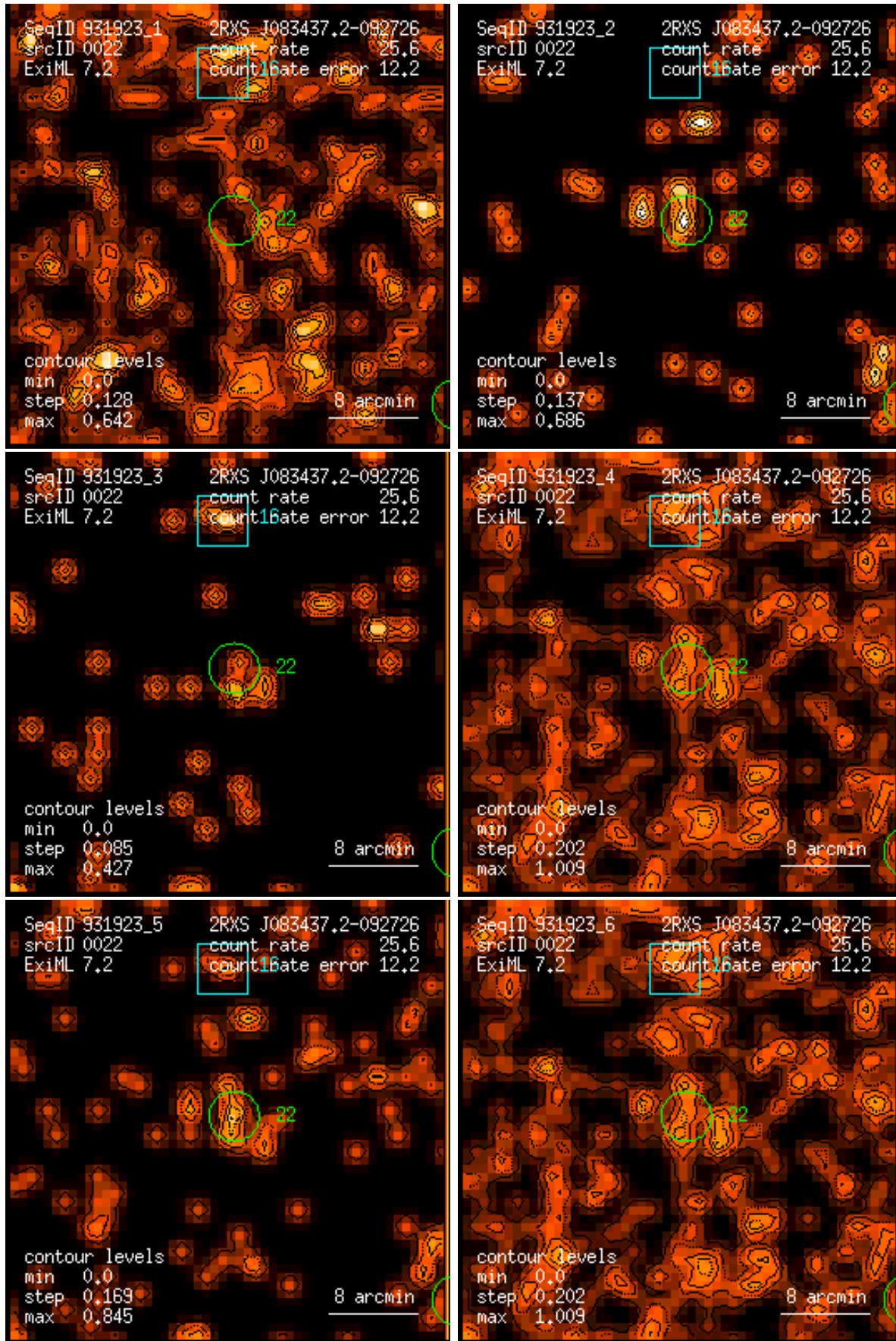
Figure 22: RASS 931923: detection 0022: band rate images, Gaussian filter: (1) PSPC channels 11 – 41, (2) 52 – 90, (3) 91 – 201, (4) 11 – 235, (5) 52 – 201, (6) 11 – 201. Broad band rates in counts/ks. Band rate contour levels in counts/ks/arcmin 2 .
