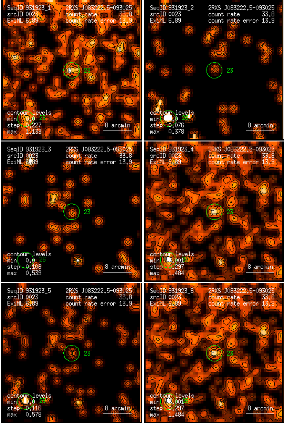
Figure 23: RASS 931923: detection 0023: band rate images, Gaussian filter: (1) PSPC channels 11 – 41, (2) 52 – 90, (3) 91 – 201, (4) 11 – 235, (5) 52 – 201, (6) 11 – 201. Broad band rates in counts/ks. Band rate contour levels in counts/ks/arcmin 2 .
