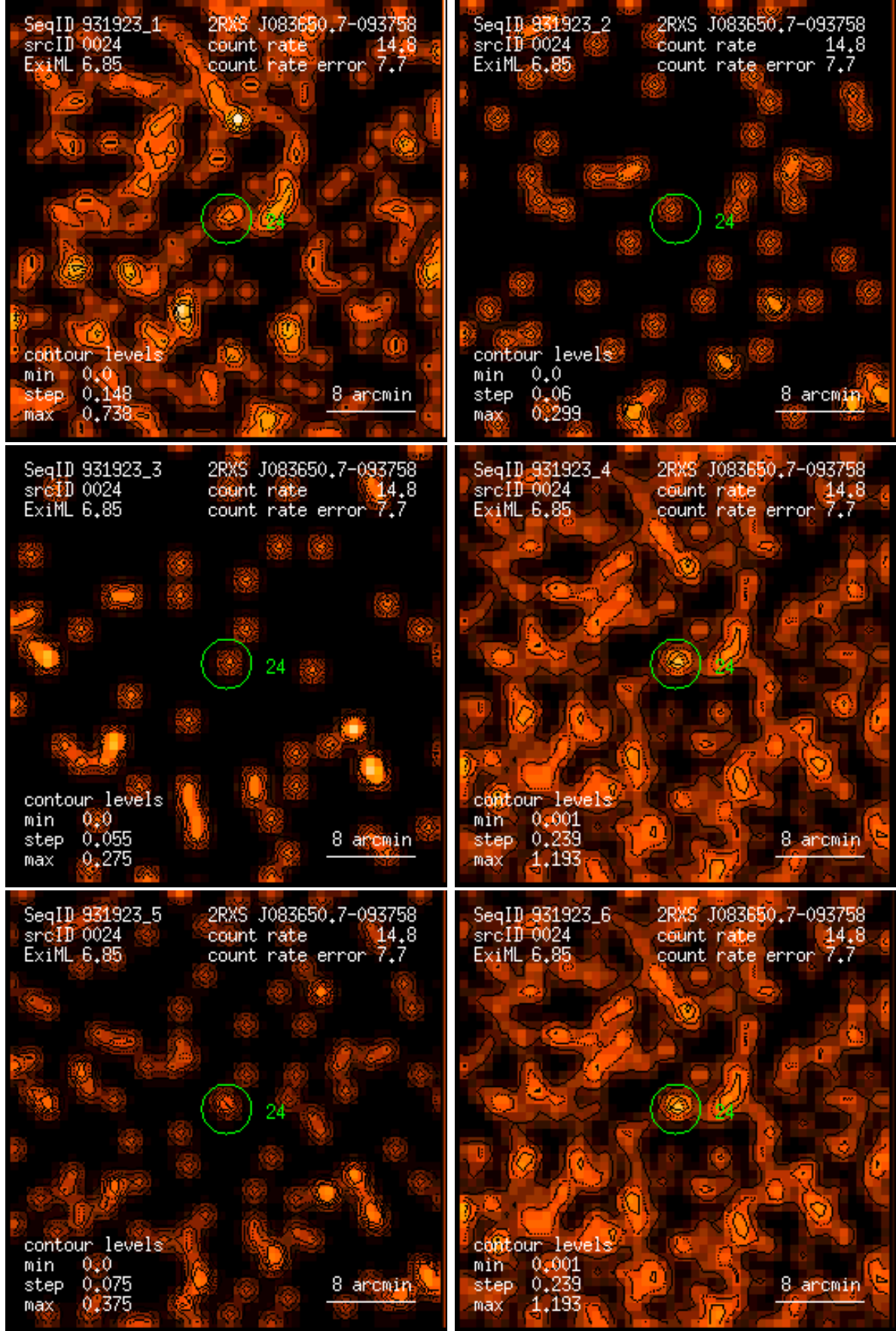
Figure 24: RASS 931923: detection 0024: band rate images, Gaussian filter: (1) PSPC channels 11 – 41, (2) 52 – 90, (3) 91 – 201, (4) 11 – 235, (5) 52 – 201, (6) 11 – 201. Broad band rates in counts/ks. Band rate contour levels in counts/ks/arcmin 2 .
