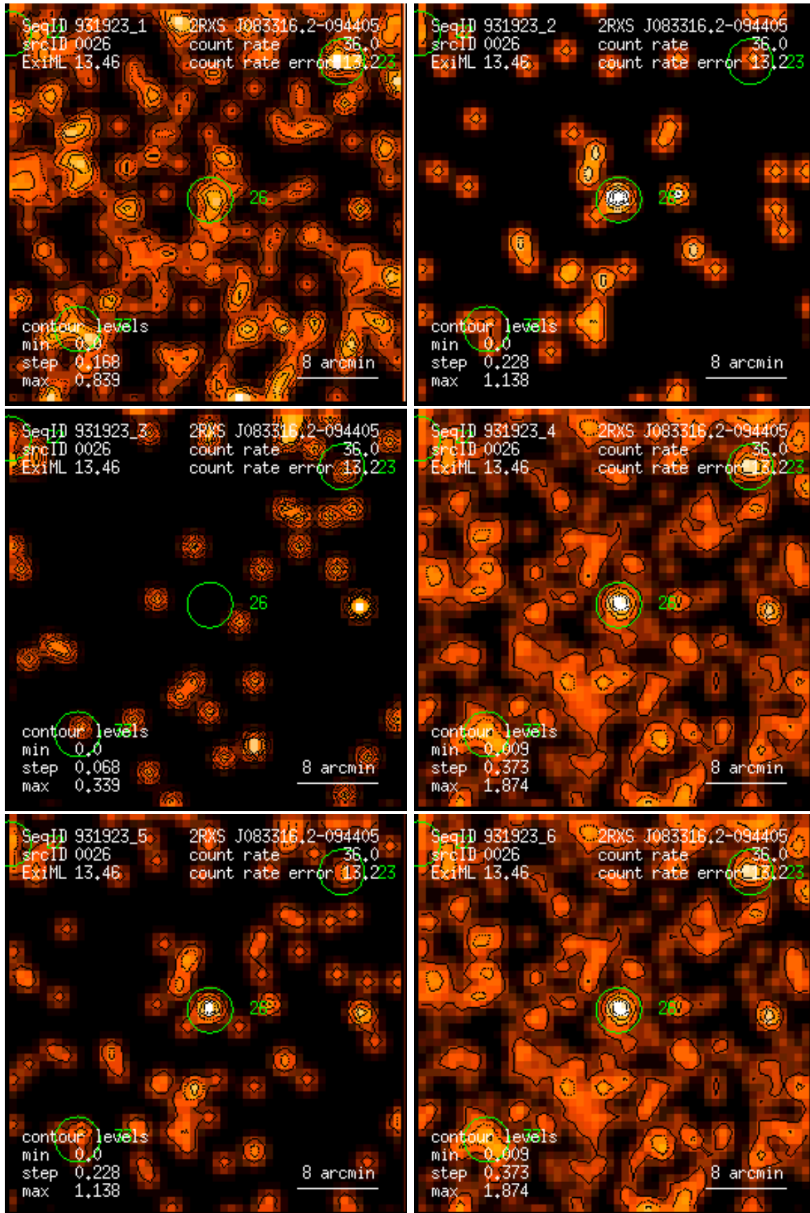
Figure 26: RASS 931923: detection 0026: band rate images, Gaussian filter: (1) PSPC channels 11 – 41, (2) 52 – 90, (3) 91 – 201, (4) 11 – 235, (5) 52 – 201, (6) 11 – 201. Broad band rates in counts/ks. Band rate contour levels in counts/ks/arcmin 2 .
