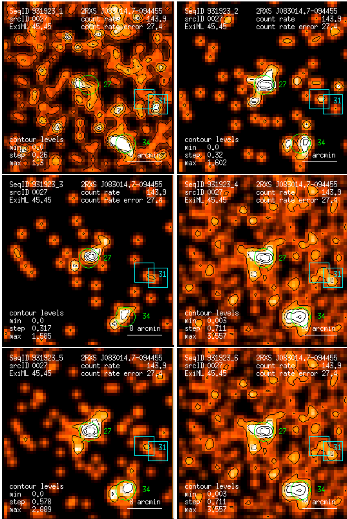
Figure 27: RASS 931923: detection 0027: band rate images, Gaussian filter: (1) PSPC channels 11 – 41, (2) 52 – 90, (3) 91 – 201, (4) 11 – 235, (5) 52 – 201, (6) 11 – 201. Broad band rates in counts/ks. Band rate contour levels in counts/ks/arcmin 2 .
