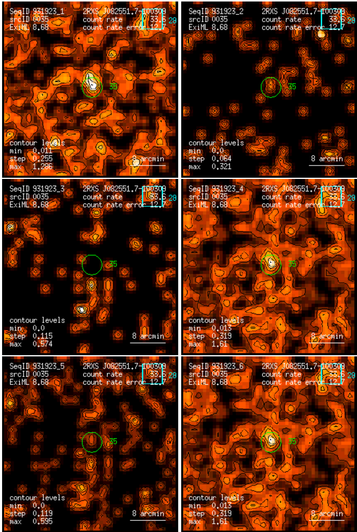
Figure 35: RASS 931923: detection 0035: band rate images, Gaussian filter: (1) PSPC channels 11 – 41, (2) 52 – 90, (3) 91 – 201, (4) 11 – 235, (5) 52 – 201, (6) 11 – 201. Broad band rates in counts/ks. Band rate contour levels in counts/ks/arcmin 2 .
