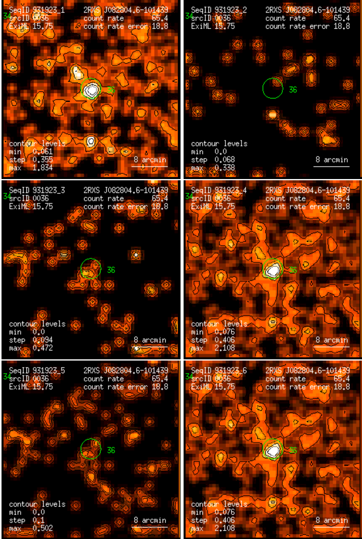
Figure 36: RASS 931923: detection 0036: band rate images, Gaussian filter: (1) PSPC channels 11 – 41, (2) 52 – 90, (3) 91 – 201, (4) 11 – 235, (5) 52 – 201, (6) 11 – 201. Broad band rates in counts/ks. Band rate contour levels in counts/ks/arcmin 2 .
