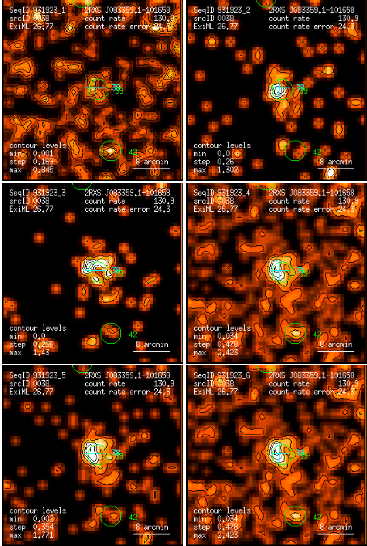
Figure 38: RASS 931923: detection 0038: band rate images, Gaussian filter: (1) PSPC channels 11 – 41, (2) 52 – 90, (3) 91 – 201, (4) 11 – 235, (5) 52 – 201, (6) 11 – 201. Broad band rates in counts/ks. Band rate contour levels in counts/ks/arcmin 2 .
