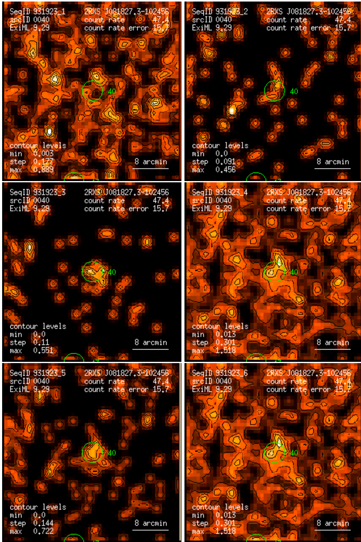
Figure 40: RASS 931923: detection 0040: band rate images, Gaussian filter: (1) PSPC channels 11 – 41, (2) 52 – 90, (3) 91 – 201, (4) 11 – 235, (5) 52 – 201, (6) 11 – 201. Broad band rates in counts/ks. Band rate contour levels in counts/ks/arcmin 2 .
