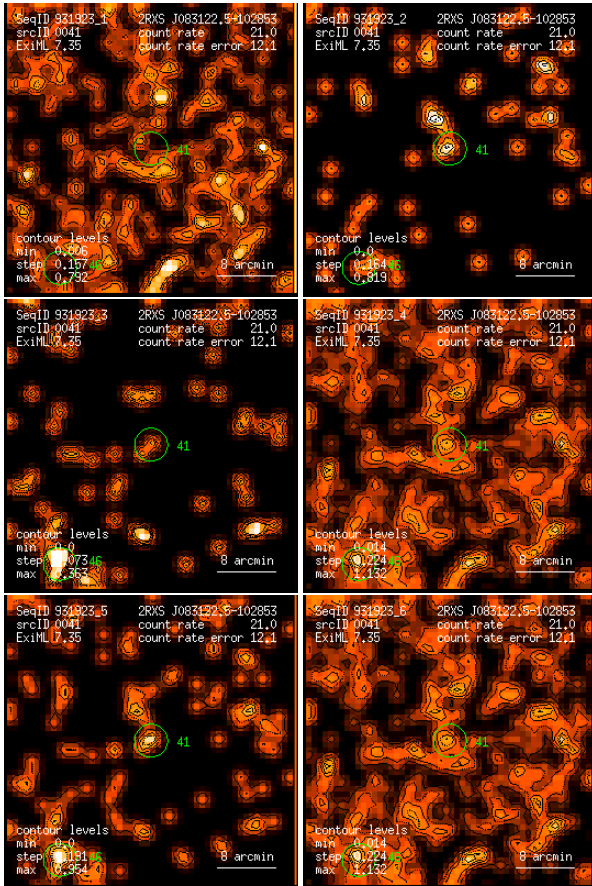
Figure 41: RASS 931923: detection 0041: band rate images, Gaussian filter: (1) PSPC channels 11 – 41, (2) 52 – 90, (3) 91 – 201, (4) 11 – 235, (5) 52 – 201, (6) 11 – 201. Broad band rates in counts/ks. Band rate contour levels in counts/ks/arcmin 2 .
