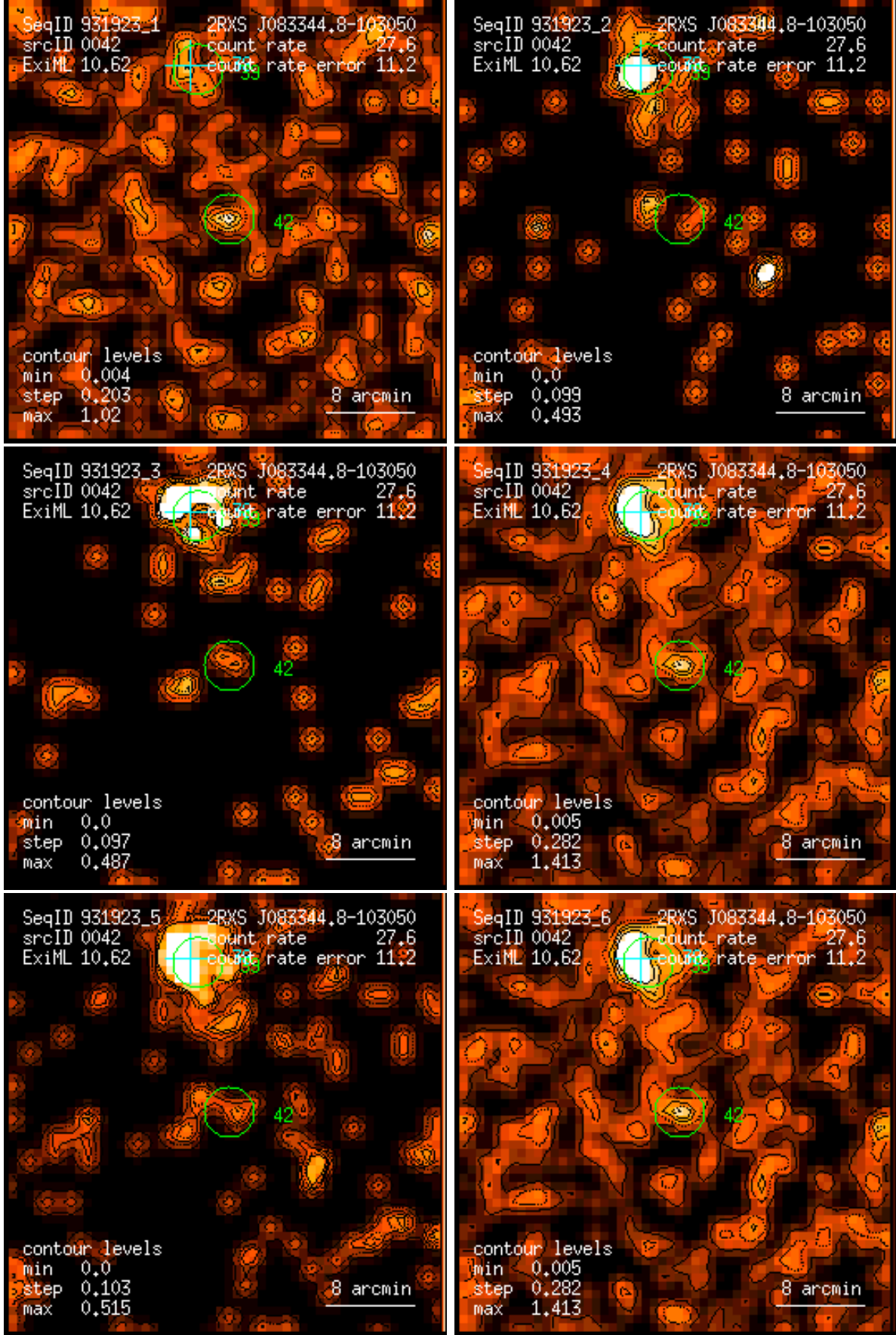
Figure 42: RASS 931923: detection 0042: band rate images, Gaussian filter: (1) PSPC channels 11 – 41, (2) 52 – 90, (3) 91 – 201, (4) 11 – 235, (5) 52 – 201, (6) 11 – 201. Broad band rates in counts/ks. Band rate contour levels in counts/ks/arcmin 2 .
