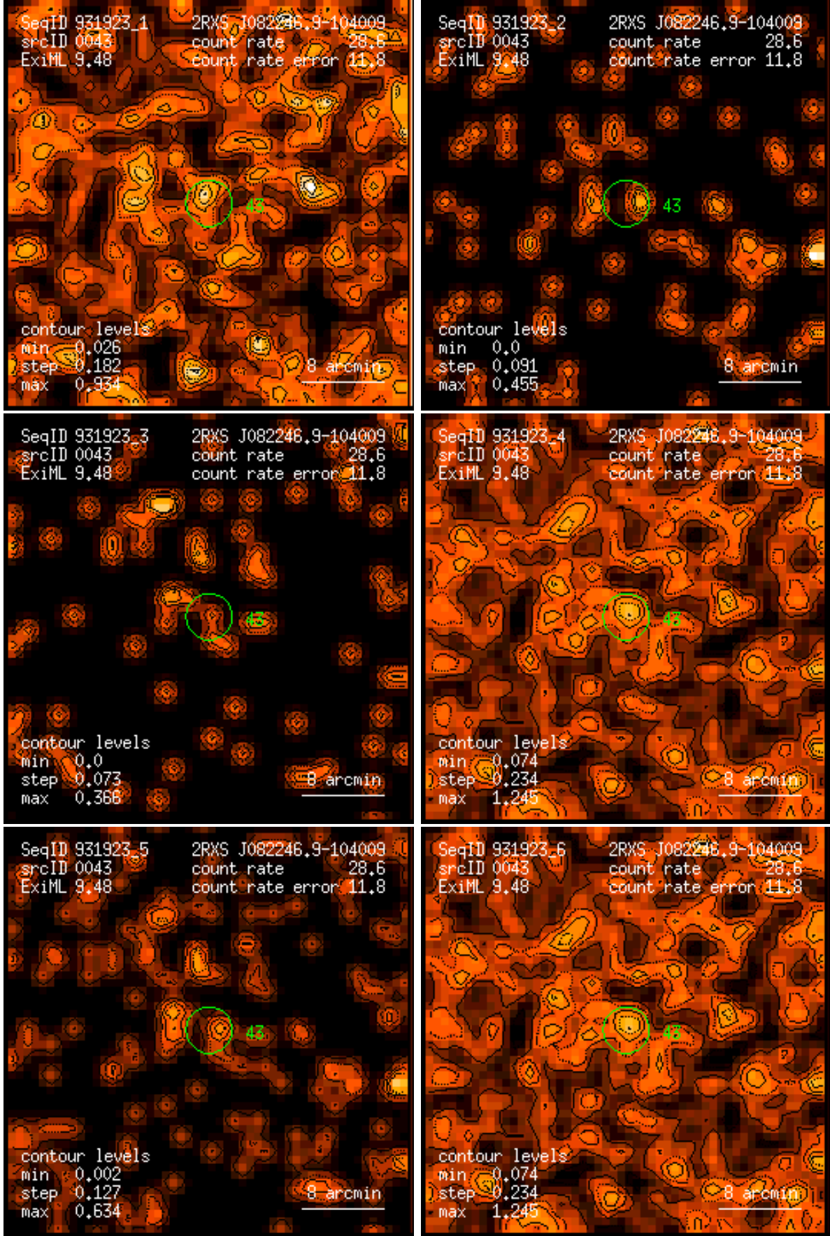
Figure 43: RASS 931923: detection 0043: band rate images, Gaussian filter: (1) PSPC channels 11 – 41, (2) 52 – 90, (3) 91 – 201, (4) 11 – 235, (5) 52 – 201, (6) 11 – 201. Broad band rates in counts/ks. Band rate contour levels in counts/ks/arcmin 2 .
