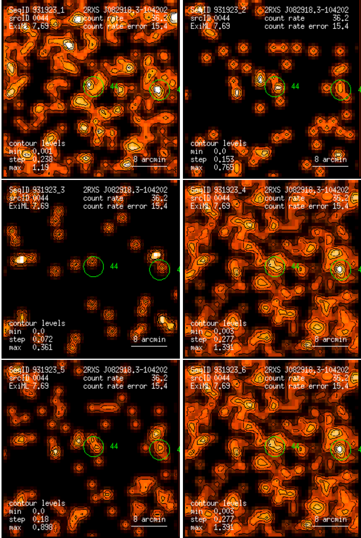
Figure 44: RASS 931923: detection 0044: band rate images, Gaussian filter: (1) PSPC channels 11 – 41, (2) 52 – 90, (3) 91 – 201, (4) 11 – 235, (5) 52 – 201, (6) 11 – 201. Broad band rates in counts/ks. Band rate contour levels in counts/ks/arcmin 2 .
