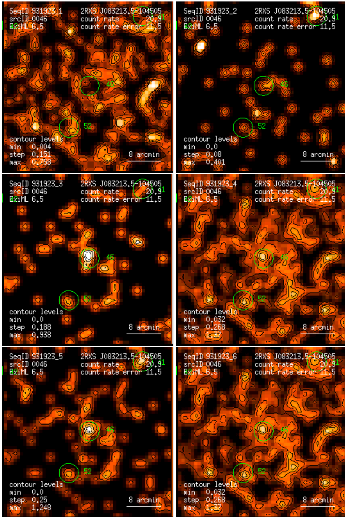
Figure 46: RASS 931923: detection 0046: band rate images, Gaussian filter: (1) PSPC channels 11 – 41, (2) 52 – 90, (3) 91 – 201, (4) 11 – 235, (5) 52 – 201, (6) 11 – 201. Broad band rates in counts/ks. Band rate contour levels in counts/ks/arcmin 2 .
