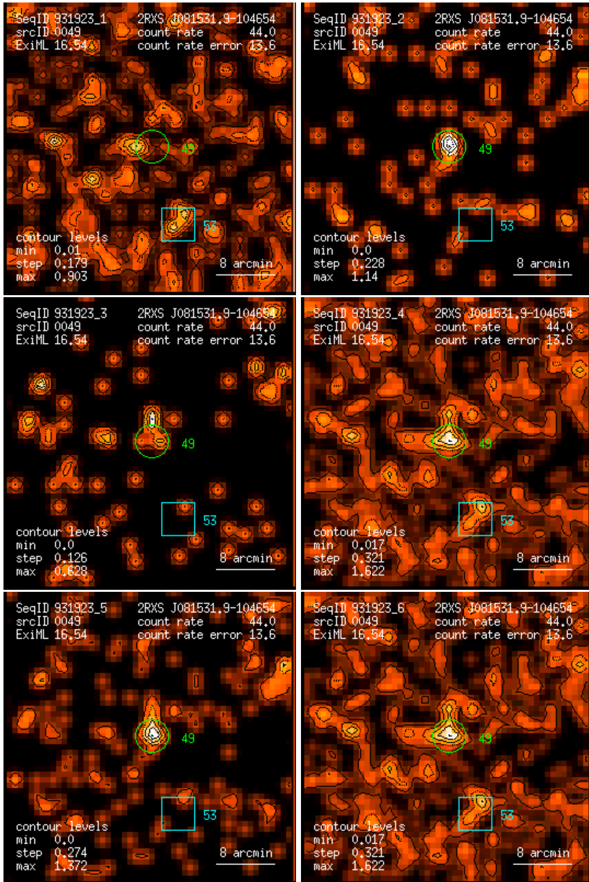
Figure 49: RASS 931923: detection 0049: band rate images, Gaussian filter: (1) PSPC channels 11 – 41, (2) 52 – 90, (3) 91 – 201, (4) 11 – 235, (5) 52 – 201, (6) 11 – 201. Broad band rates in counts/ks. Band rate contour levels in counts/ks/arcmin 2 .
