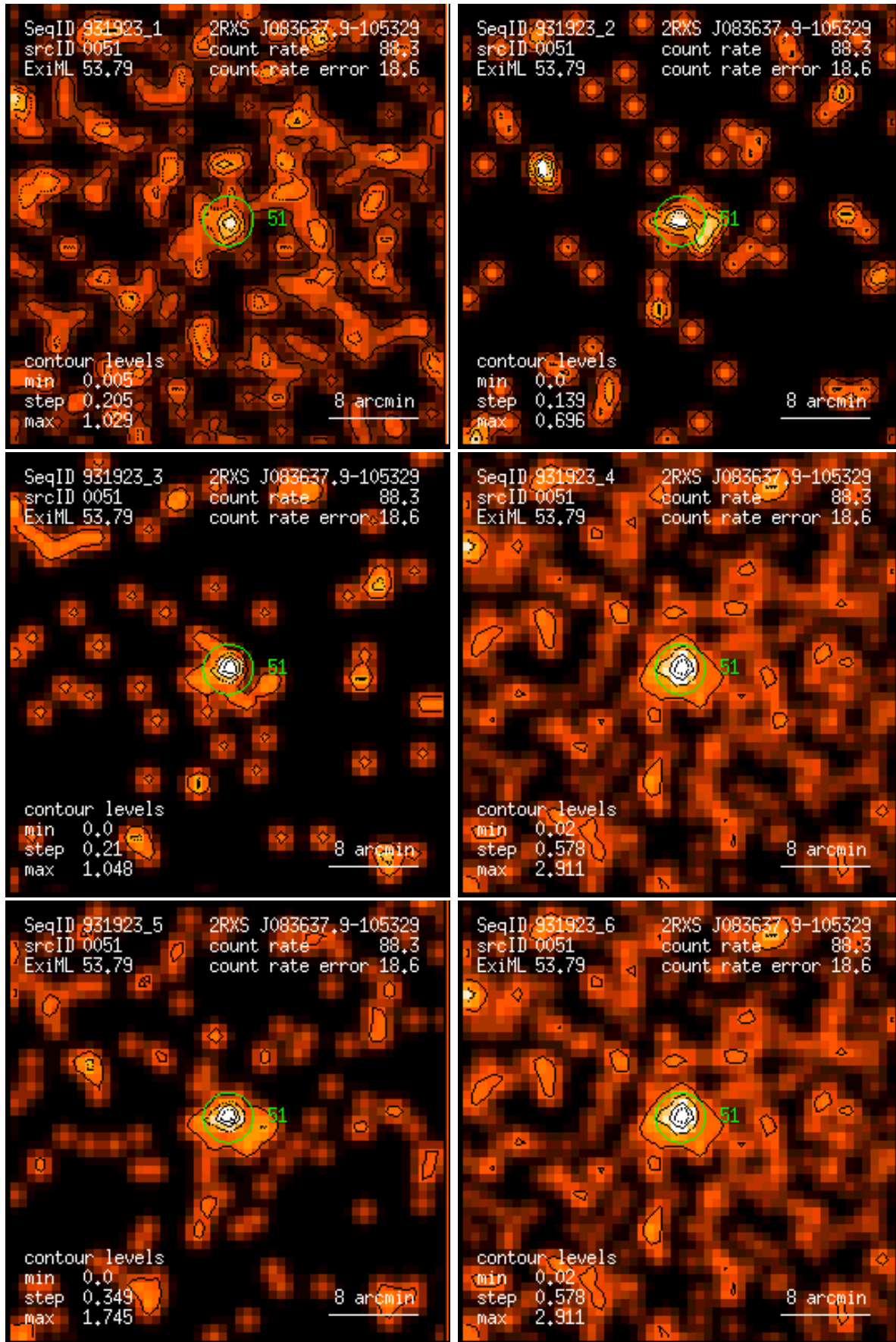
Figure 51: RASS 931923: detection 0051: band rate images, Gaussian filter: (1) PSPC channels 11 – 41, (2) 52 – 90, (3) 91 – 201, (4) 11 – 235, (5) 52 – 201, (6) 11 – 201. Broad band rates in counts/ks. Band rate contour levels in counts/ks/arcmin 2 .
