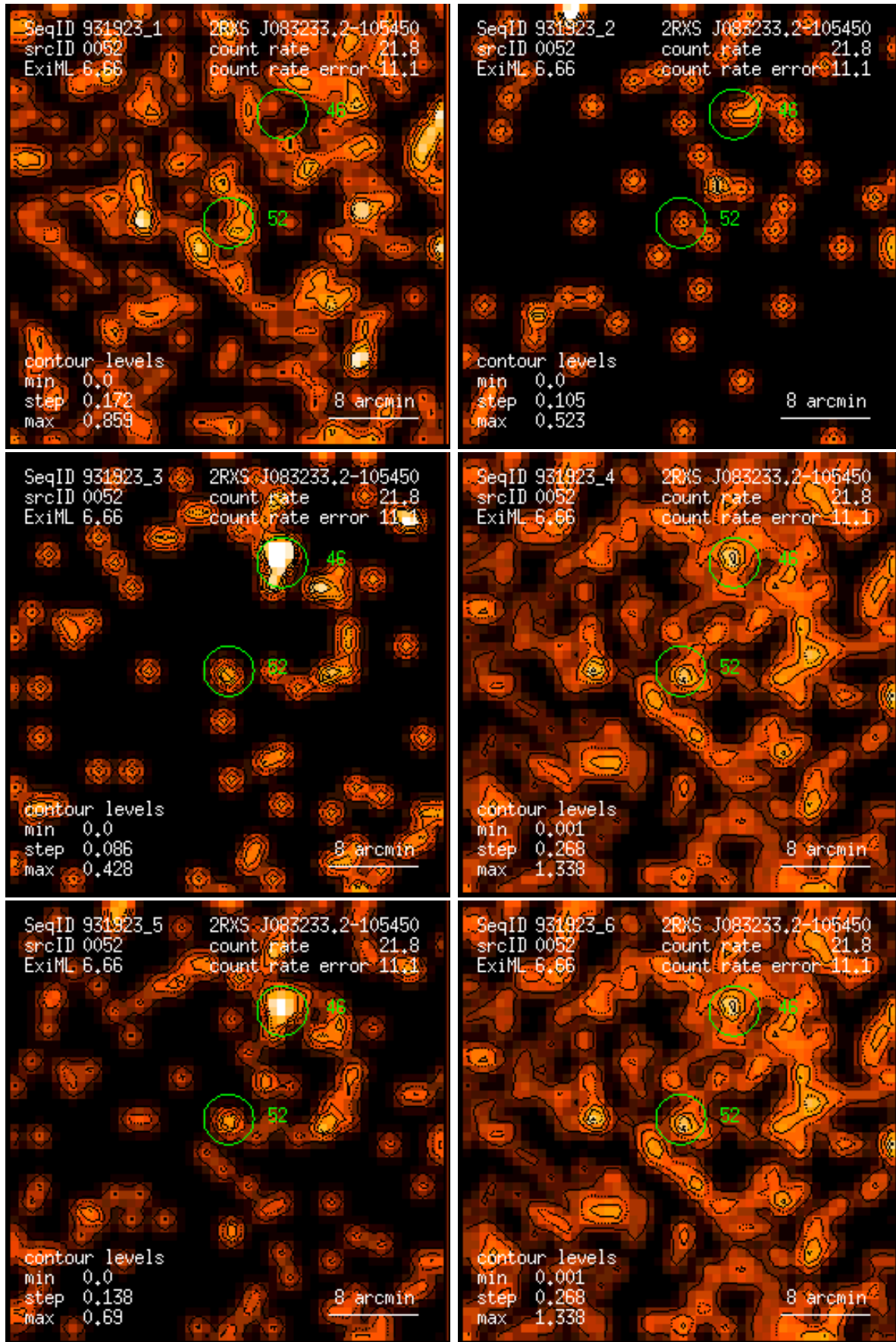
Figure 52: RASS 931923: detection 0052: band rate images, Gaussian filter: (1) PSPC channels 11 – 41, (2) 52 – 90, (3) 91 – 201, (4) 11 – 235, (5) 52 – 201, (6) 11 – 201. Broad band rates in counts/ks. Band rate contour levels in counts/ks/arcmin 2 .
