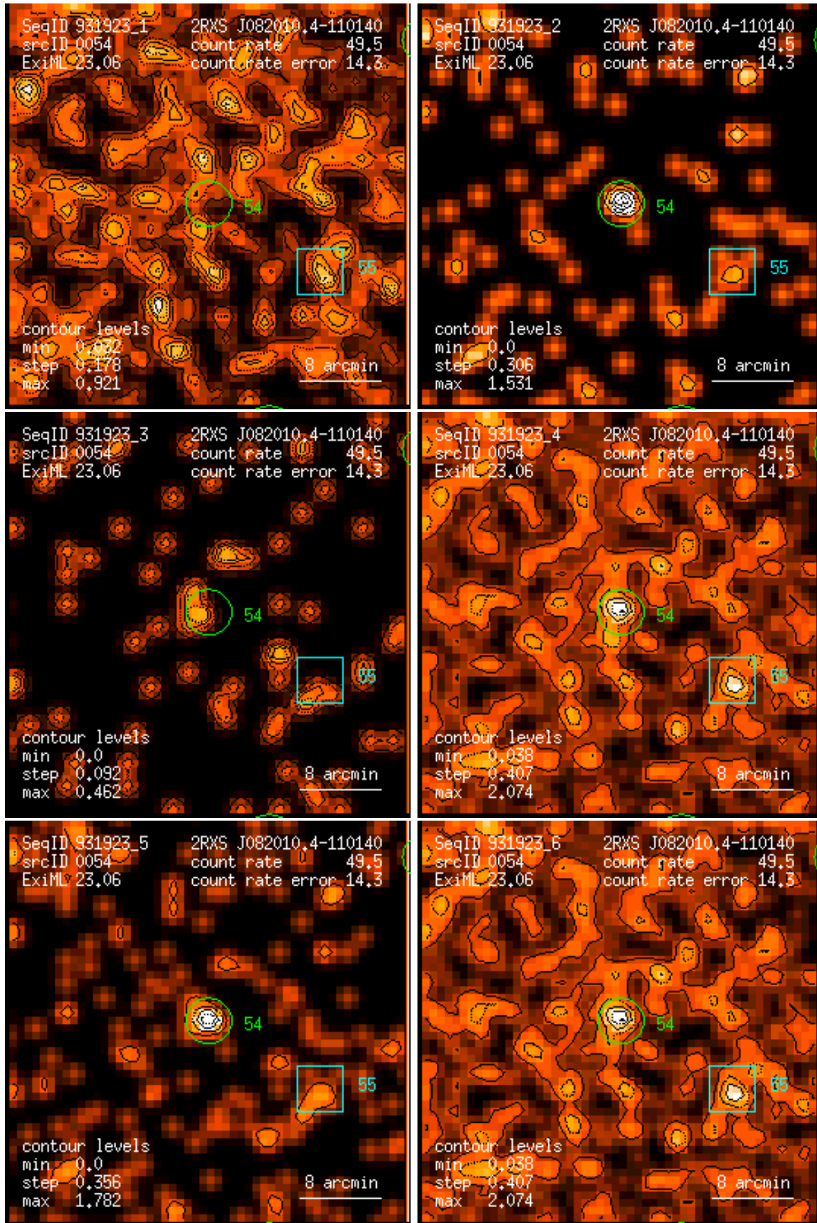
Figure 54: RASS 931923: detection 0054: band rate images, Gaussian filter: (1) PSPC channels 11 – 41, (2) 52 – 90, (3) 91 – 201, (4) 11 – 235, (5) 52 – 201, (6) 11 – 201. Broad band rates in counts/ks. Band rate contour levels in counts/ks/arcmin 2 .
