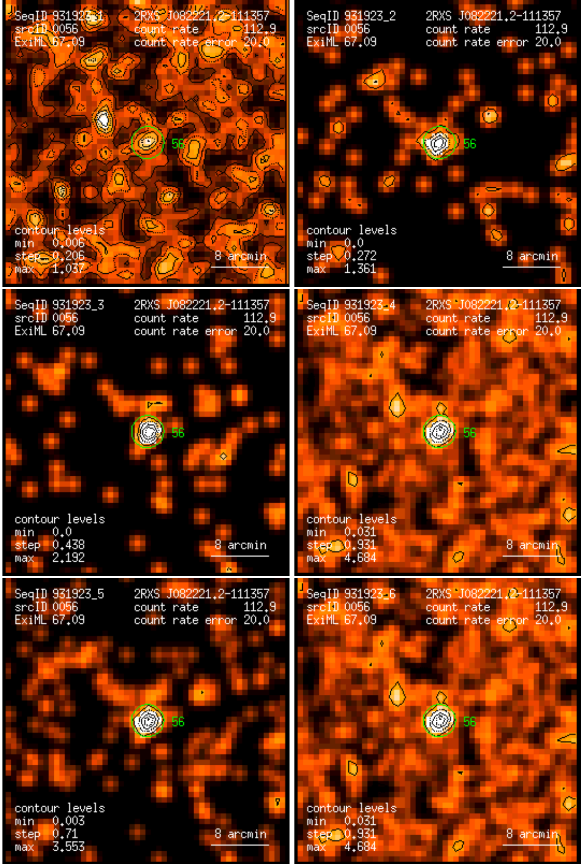
Figure 56: RASS 931923: detection 0056: band rate images, Gaussian filter: (1) PSPC channels 11 – 41, (2) 52 – 90, (3) 91 – 201, (4) 11 – 235, (5) 52 – 201, (6) 11 – 201. Broad band rates in counts/ks. Band rate contour levels in counts/ks/arcmin 2 .
