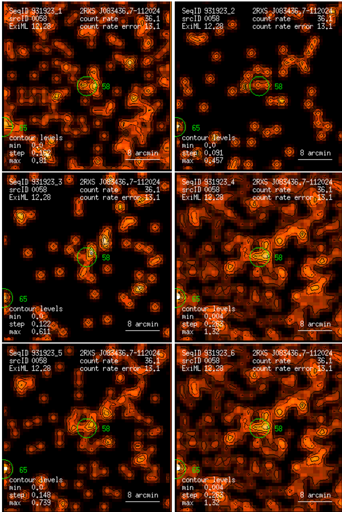
Figure 58: RASS 931923: detection 0058: band rate images, Gaussian filter: (1) PSPC channels 11 – 41, (2) 52 – 90, (3) 91 – 201, (4) 11 – 235, (5) 52 – 201, (6) 11 – 201. Broad band rates in counts/ks. Band rate contour levels in counts/ks/arcmin 2 .
