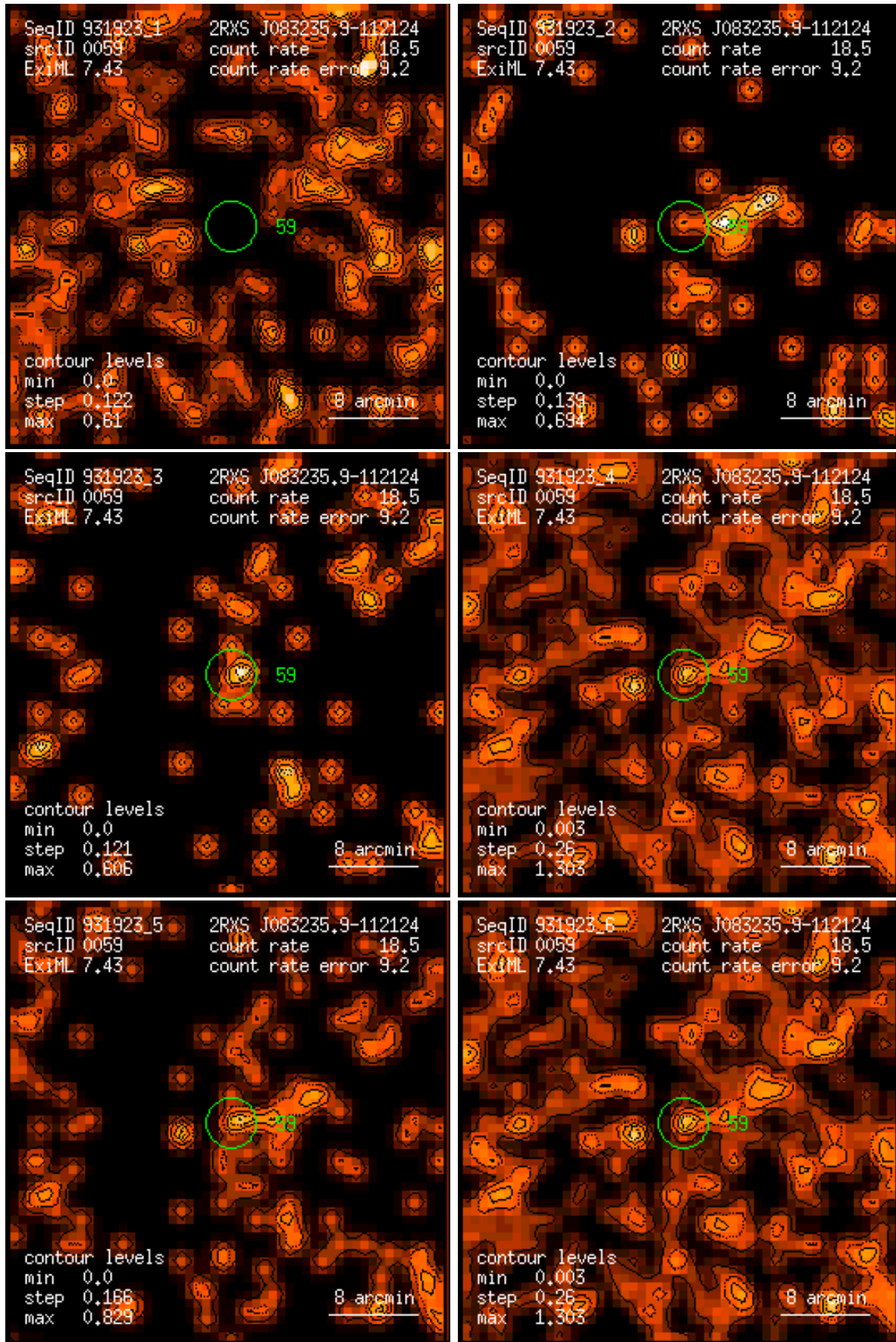
Figure 59: RASS 931923: detection 0059: band rate images, Gaussian filter: (1) PSPC channels 11 – 41, (2) 52 – 90, (3) 91 – 201, (4) 11 – 235, (5) 52 – 201, (6) 11 – 201. Broad band rates in counts/ks. Band rate contour levels in counts/ks/arcmin 2 .
