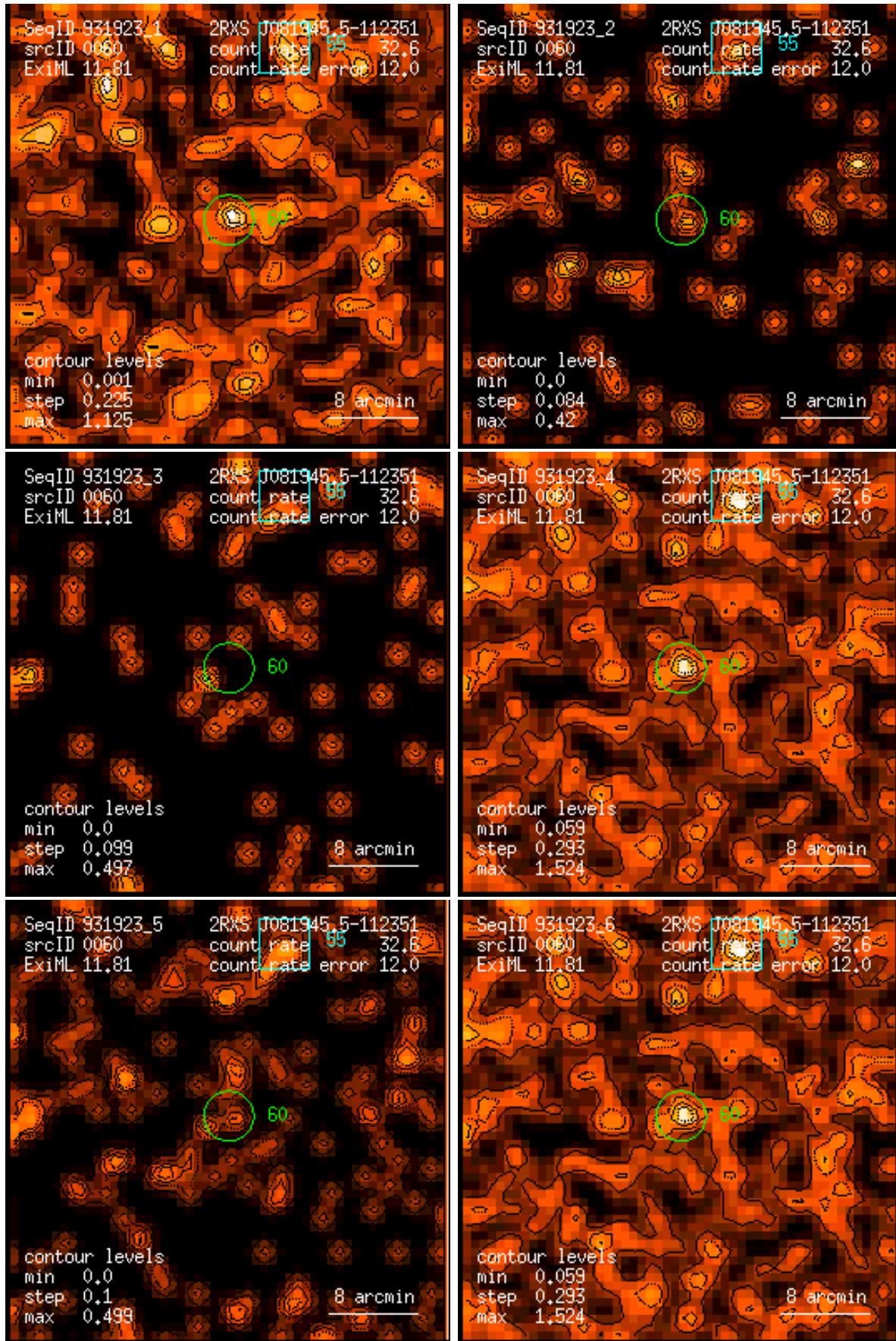
Figure 60: RASS 931923: detection 0060: band rate images, Gaussian filter: (1) PSPC channels 11 – 41, (2) 52 – 90, (3) 91 – 201, (4) 11 – 235, (5) 52 – 201, (6) 11 – 201. Broad band rates in counts/ks. Band rate contour levels in counts/ks/arcmin 2 .
