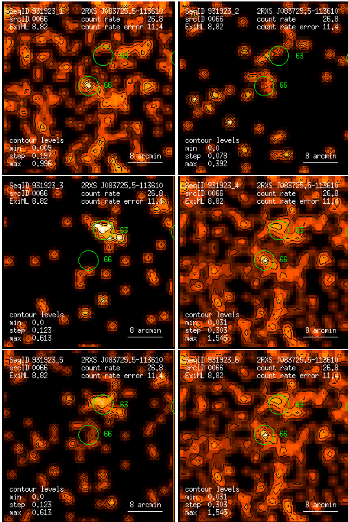
Figure 66: RASS 931923: detection 0066: band rate images, Gaussian filter: (1) PSPC channels 11 – 41, (2) 52 – 90, (3) 91 – 201, (4) 11 – 235, (5) 52 – 201, (6) 11 – 201. Broad band rates in counts/ks. Band rate contour levels in counts/ks/arcmin 2 .
