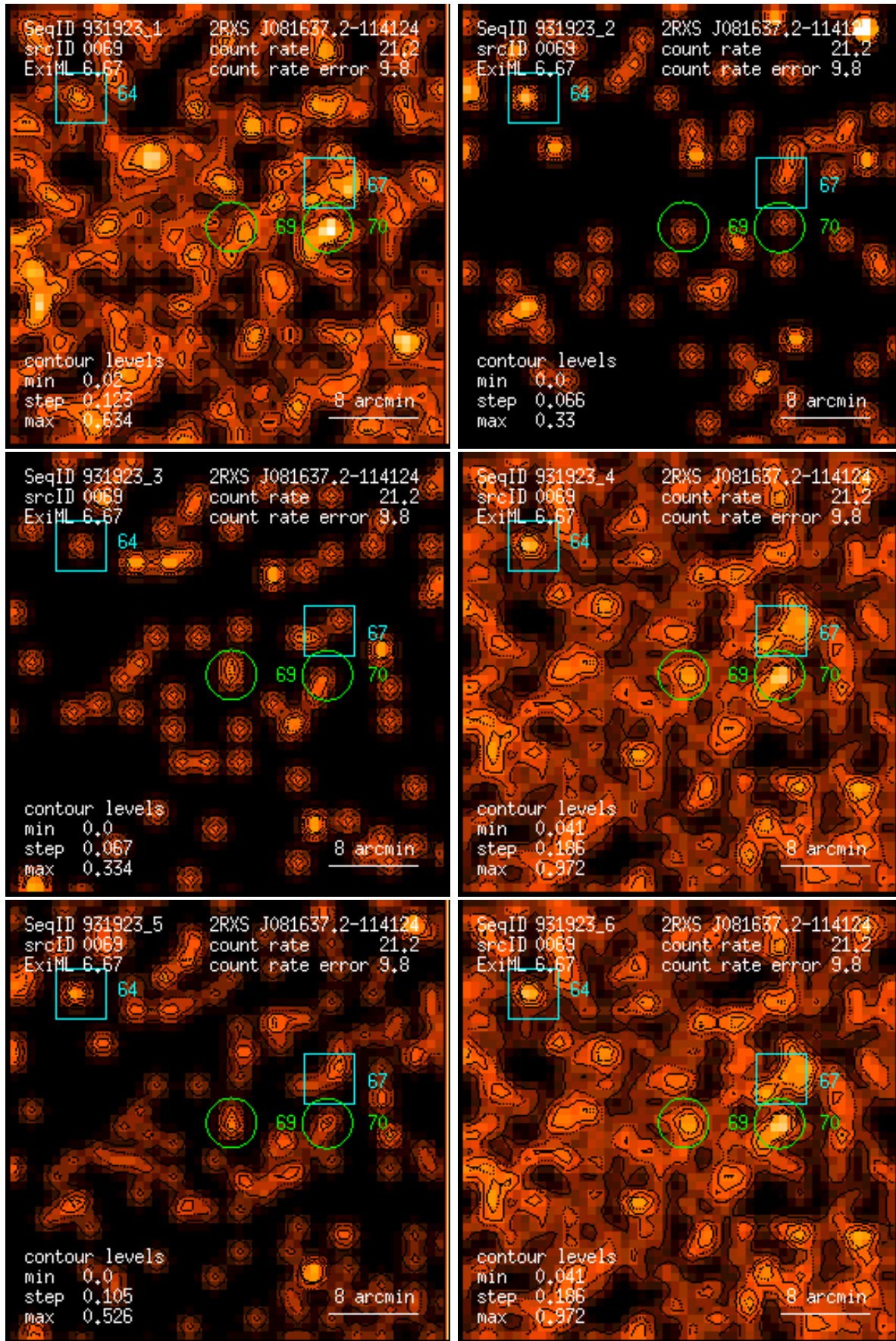
Figure 69: RASS 931923: detection 0069: band rate images, Gaussian filter: (1) PSPC channels 11 – 41, (2) 52 – 90, (3) 91 – 201, (4) 11 – 235, (5) 52 – 201, (6) 11 – 201. Broad band rates in counts/ks. Band rate contour levels in counts/ks/arcmin 2 .
