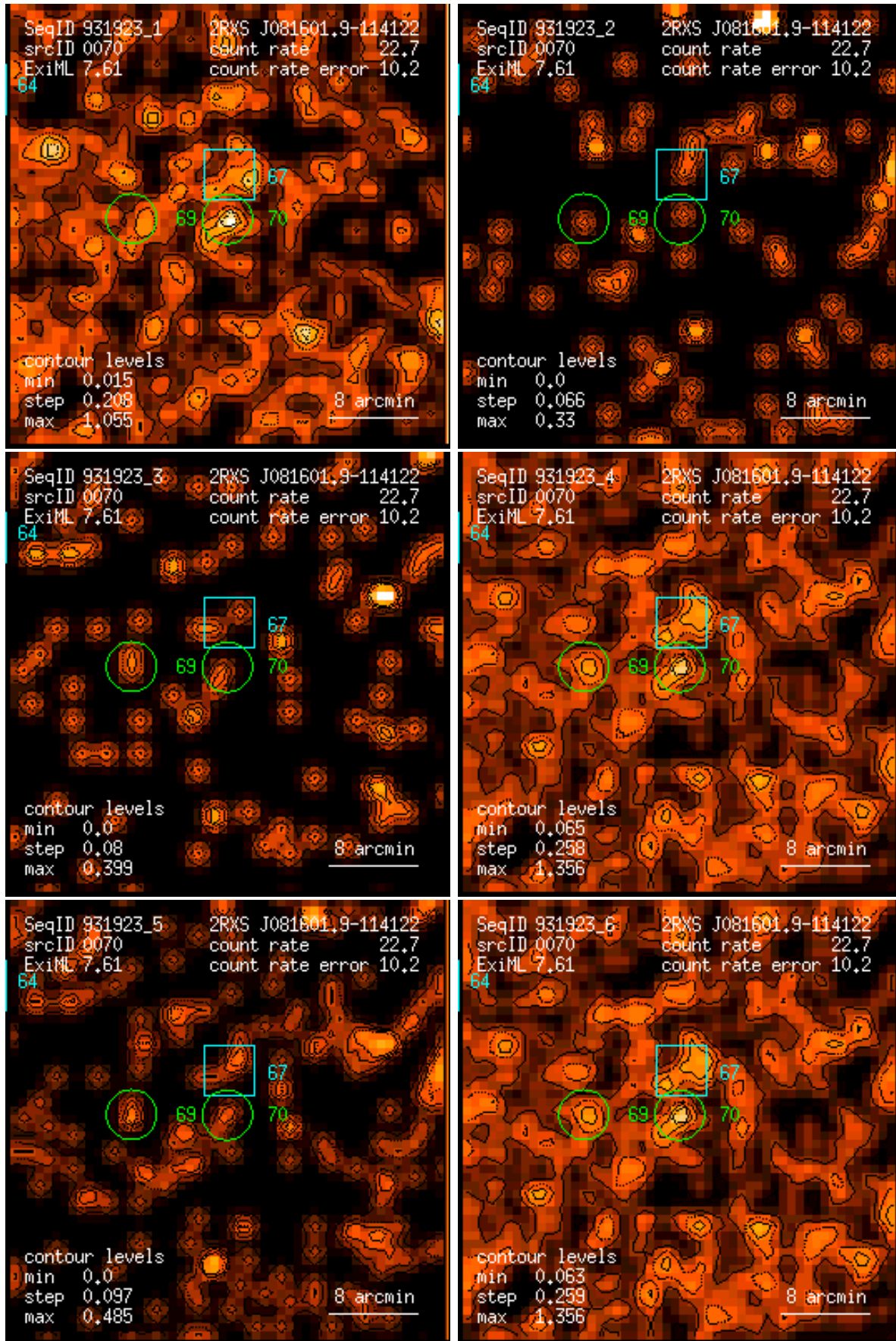
Figure 70: RASS 931923: detection 0070: band rate images, Gaussian filter: (1) PSPC channels 11 – 41, (2) 52 – 90, (3) 91 – 201, (4) 11 – 235, (5) 52 – 201, (6) 11 – 201. Broad band rates in counts/ks. Band rate contour levels in counts/ks/arcmin 2 .
