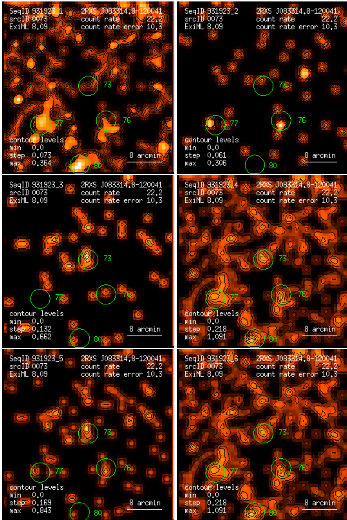
Figure 73: RASS 931923: detection 0073: band rate images, Gaussian filter: (1) PSPC channels 11 – 41, (2) 52 – 90, (3) 91 – 201, (4) 11 – 235, (5) 52 – 201, (6) 11 – 201. Broad band rates in counts/ks. Band rate contour levels in counts/ks/arcmin 2 .
