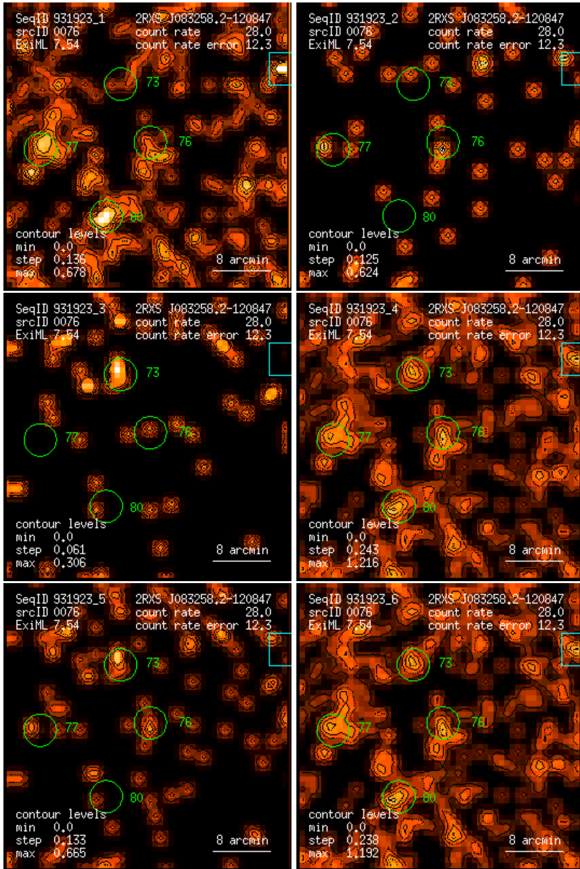
Figure 76: RASS 931923: detection 0076: band rate images, Gaussian filter: (1) PSPC channels 11 – 41, (2) 52 – 90, (3) 91 – 201, (4) 11 – 235, (5) 52 – 201, (6) 11 – 201. Broad band rates in counts/ks. Band rate contour levels in counts/ks/arcmin 2 .
