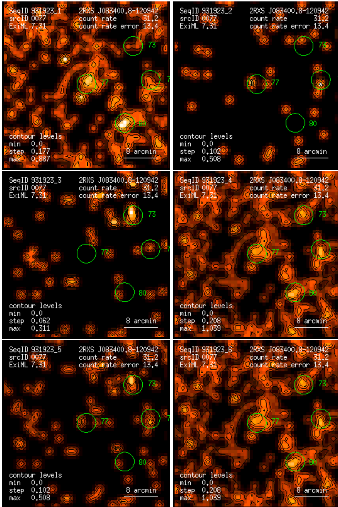
Figure 77: RASS 931923: detection 0077: band rate images, Gaussian filter: (1) PSPC channels 11 – 41, (2) 52 – 90, (3) 91 – 201, (4) 11 – 235, (5) 52 – 201, (6) 11 – 201. Broad band rates in counts/ks. Band rate contour levels in counts/ks/arcmin 2 .
