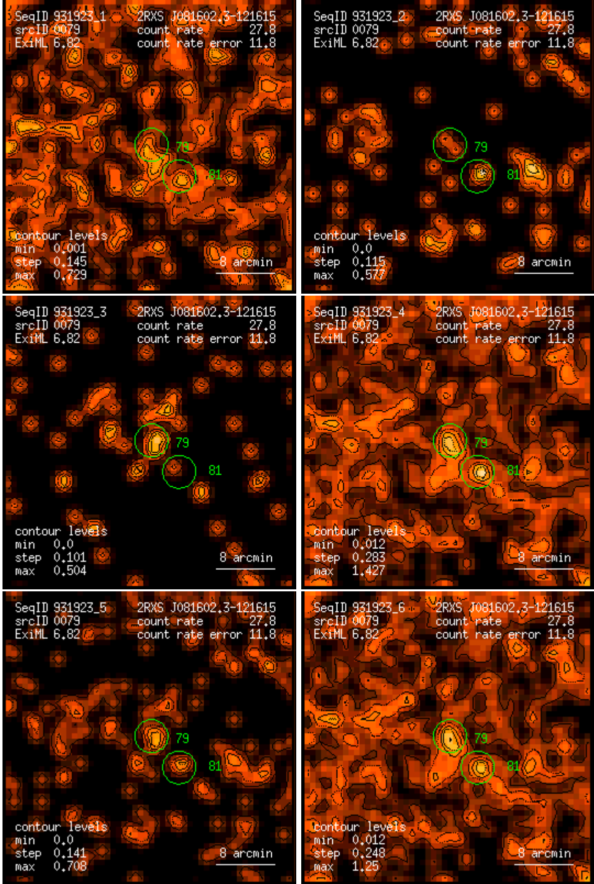
Figure 79: RASS 931923: detection 0079: band rate images, Gaussian filter: (1) PSPC channels 11 – 41, (2) 52 – 90, (3) 91 – 201, (4) 11 – 235, (5) 52 – 201, (6) 11 – 201. Broad band rates in counts/ks. Band rate contour levels in counts/ks/arcmin 2 .
