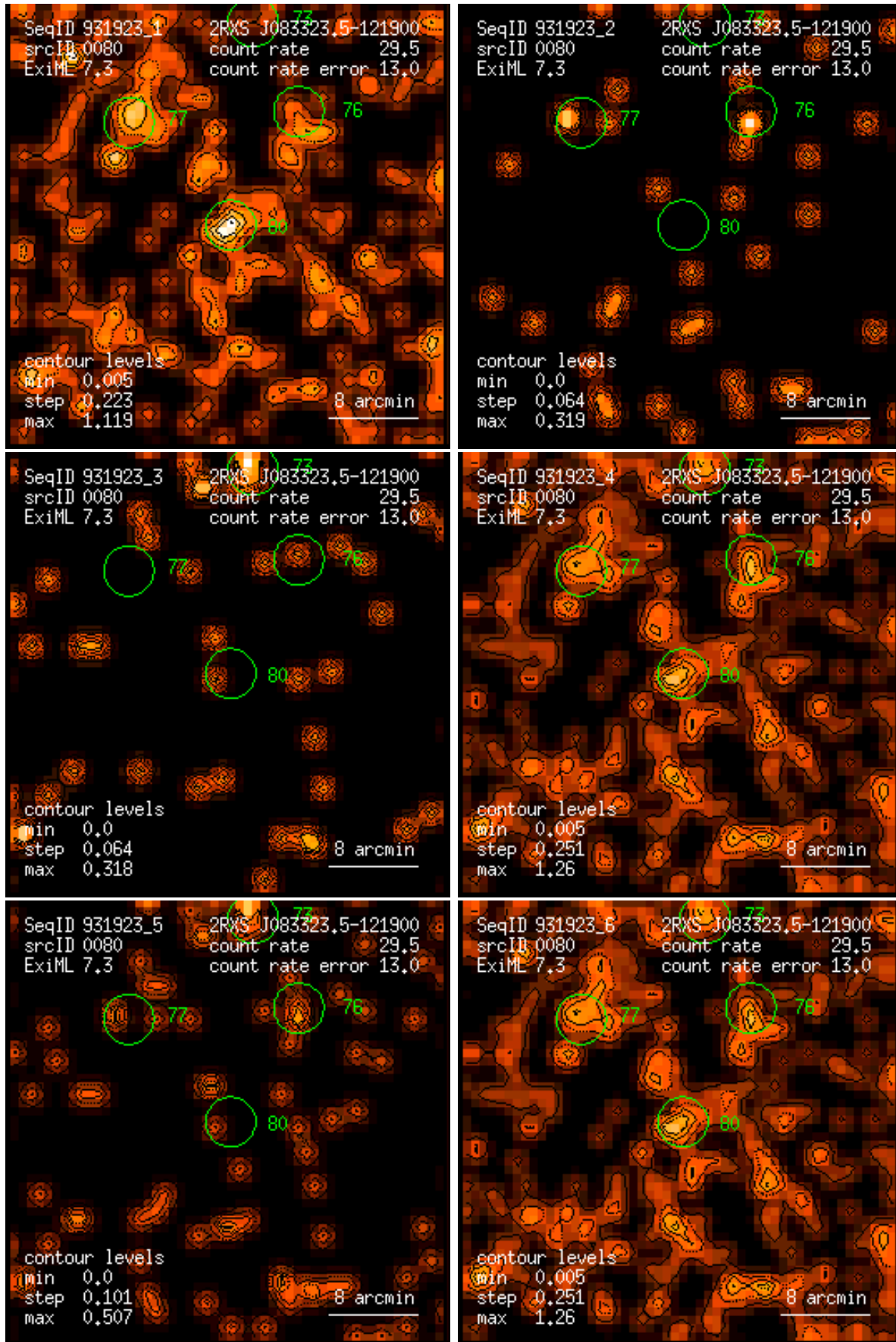
Figure 80: RASS 931923: detection 0080: band rate images, Gaussian filter: (1) PSPC channels 11 – 41, (2) 52 – 90, (3) 91 – 201, (4) 11 – 235, (5) 52 – 201, (6) 11 – 201. Broad band rates in counts/ks. Band rate contour levels in counts/ks/arcmin 2 .
