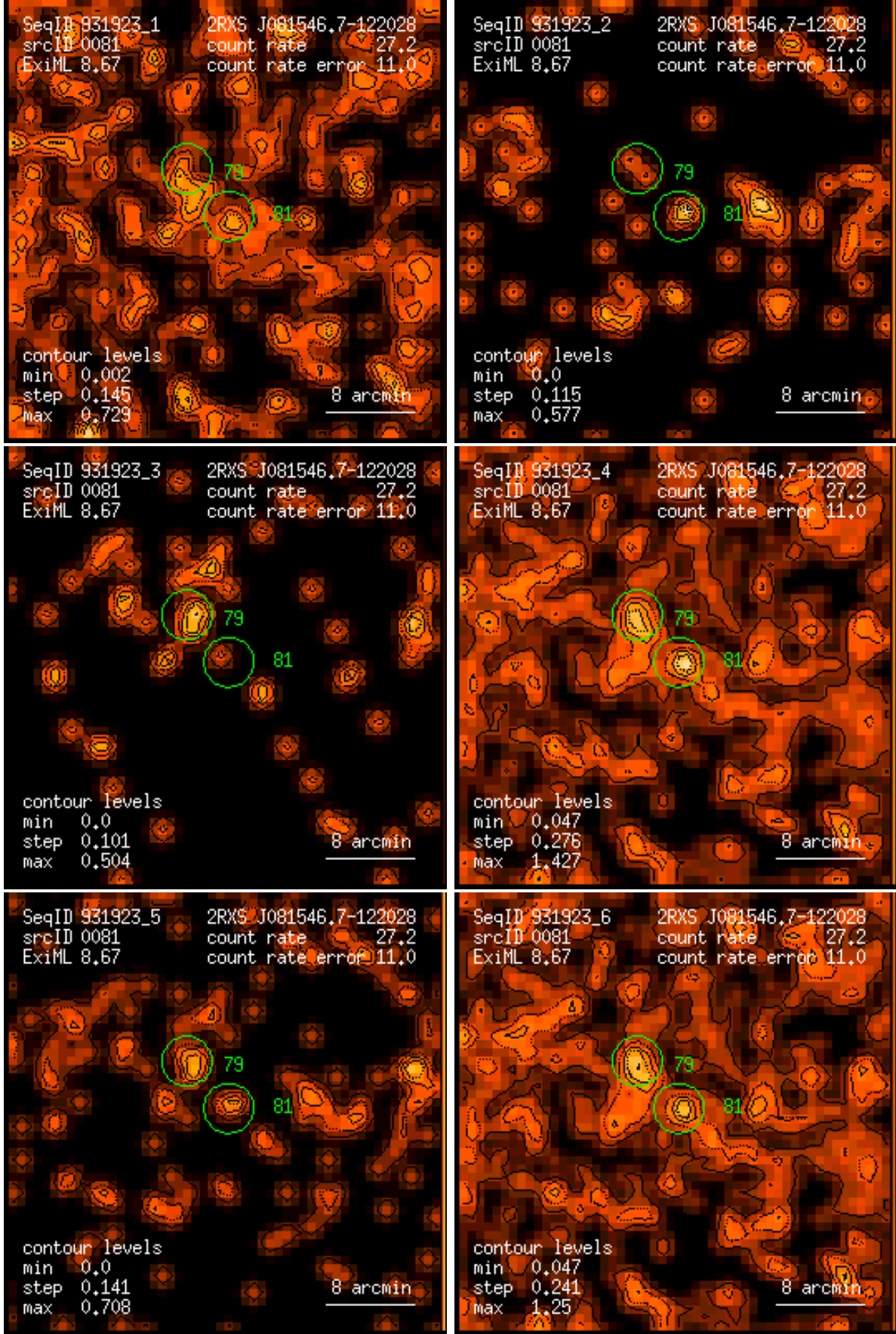
Figure 81: RASS 931923: detection 0081: band rate images, Gaussian filter: (1) PSPC channels 11 – 41, (2) 52 – 90, (3) 91 – 201, (4) 11 – 235, (5) 52 – 201, (6) 11 – 201. Broad band rates in counts/ks. Band rate contour levels in counts/ks/arcmin 2 .
