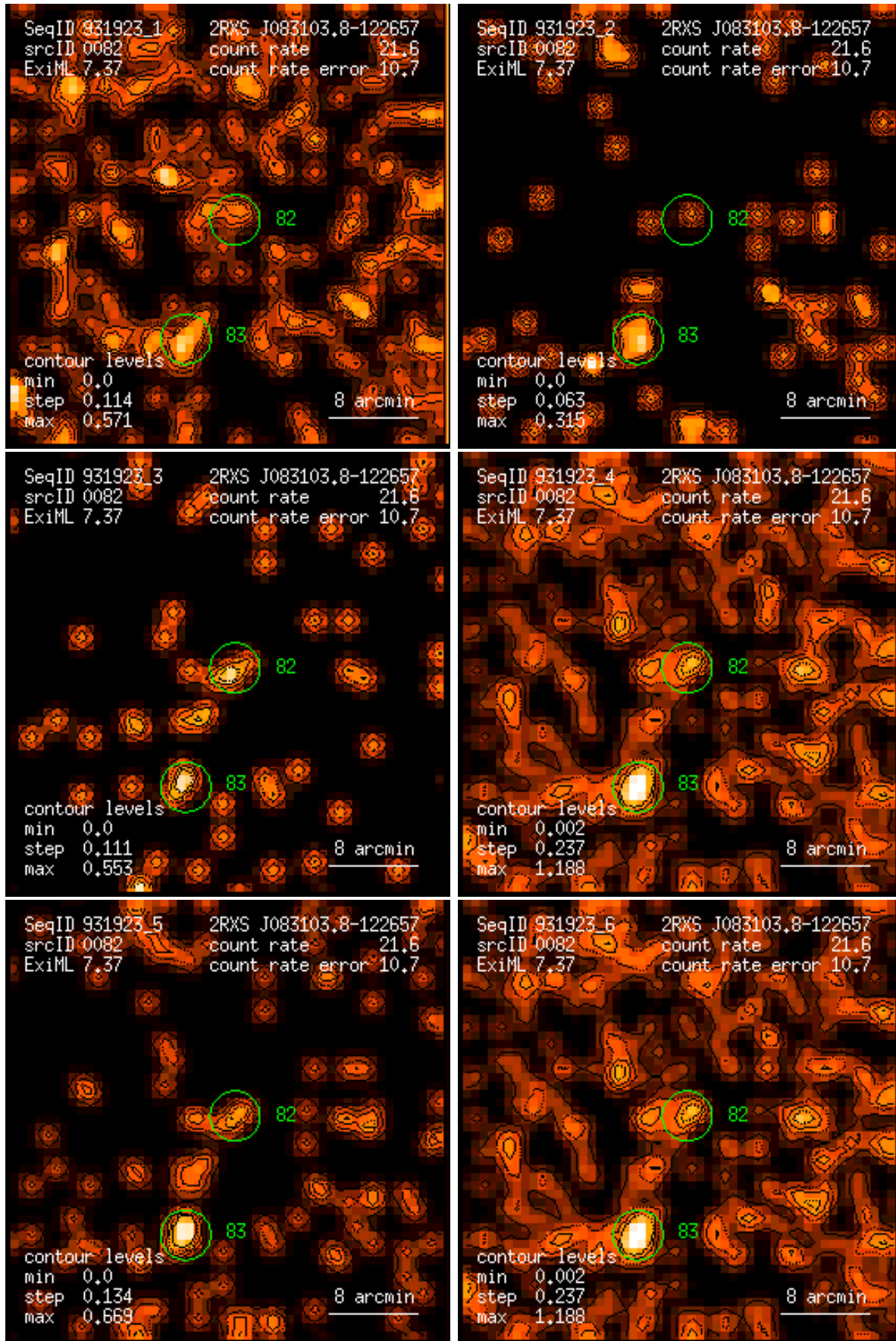
Figure 82: RASS 931923: detection 0082: band rate images, Gaussian filter: (1) PSPC channels 11 – 41, (2) 52 – 90, (3) 91 – 201, (4) 11 – 235, (5) 52 – 201, (6) 11 – 201. Broad band rates in counts/ks. Band rate contour levels in counts/ks/arcmin 2 .
