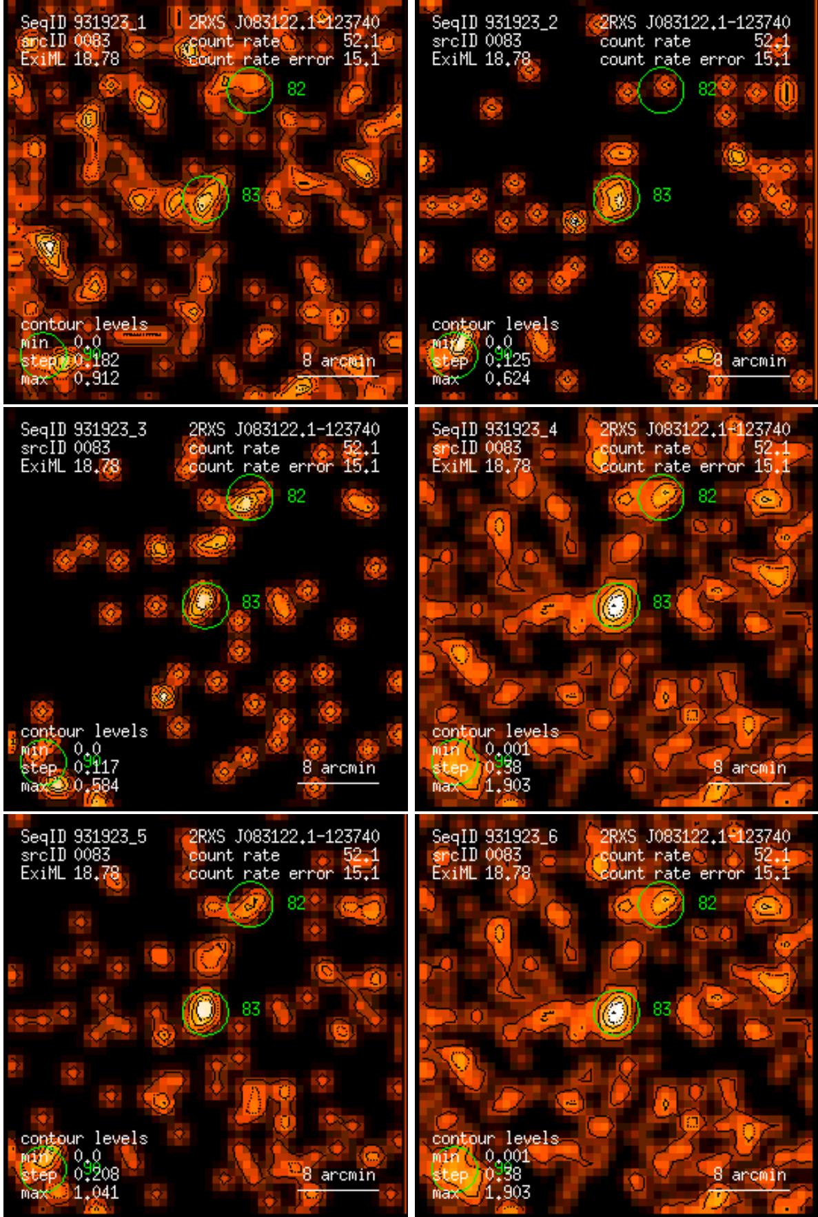
Figure 83: RASS 931923: detection 0083: band rate images, Gaussian filter: (1) PSPC channels 11 – 41, (2) 52 – 90, (3) 91 – 201, (4) 11 – 235, (5) 52 – 201, (6) 11 – 201. Broad band rates in counts/ks. Band rate contour levels in counts/ks/arcmin 2 .
